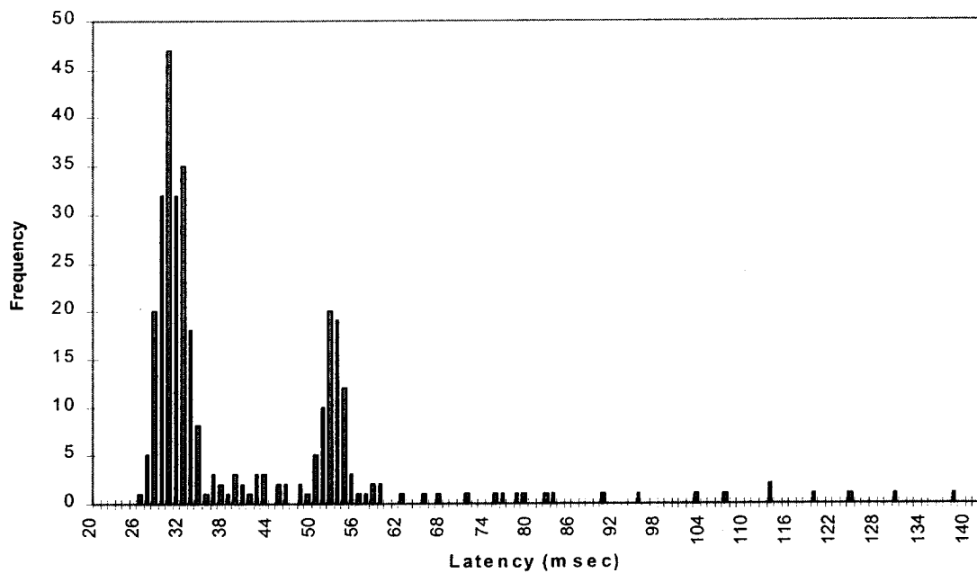
Figure 4.3.3.1-18b. Frequency Histogram of Latency of Shooter Entity State Data (before launch) Between WSSF Simulation and WSIC PDU Logger (Run #12 on 11/19/96)
