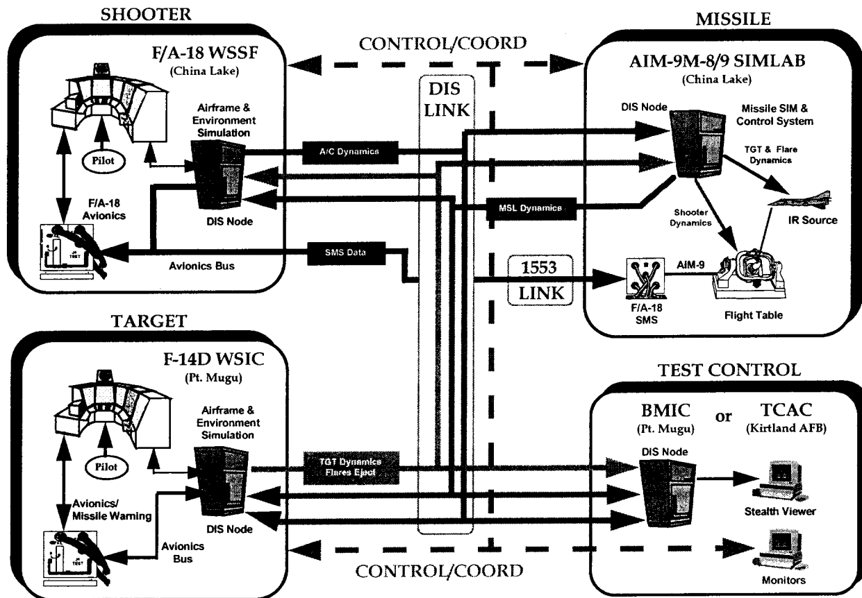
Figure 2.4.3.2-1. Linked Simulators Phase Test Configuration
