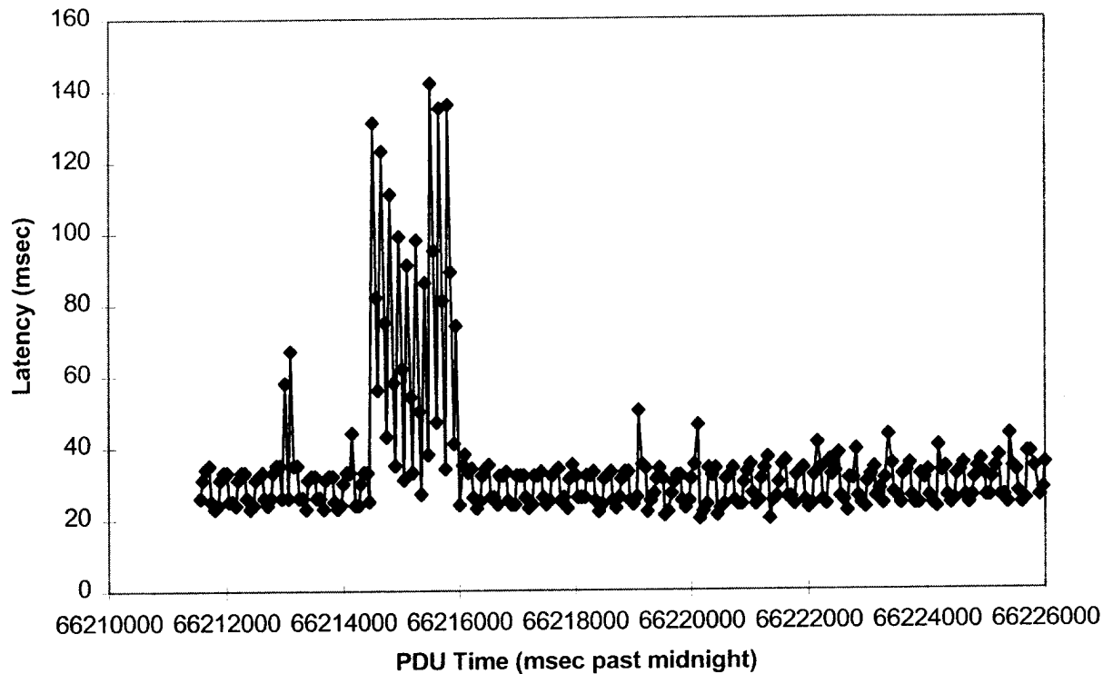
Figure 4.3.3.1-14a. Latency of Target Entity State Data (before launch) Between WSIC Simulation and WSSF PDU Logger (Run #19 on 11/19/96)
