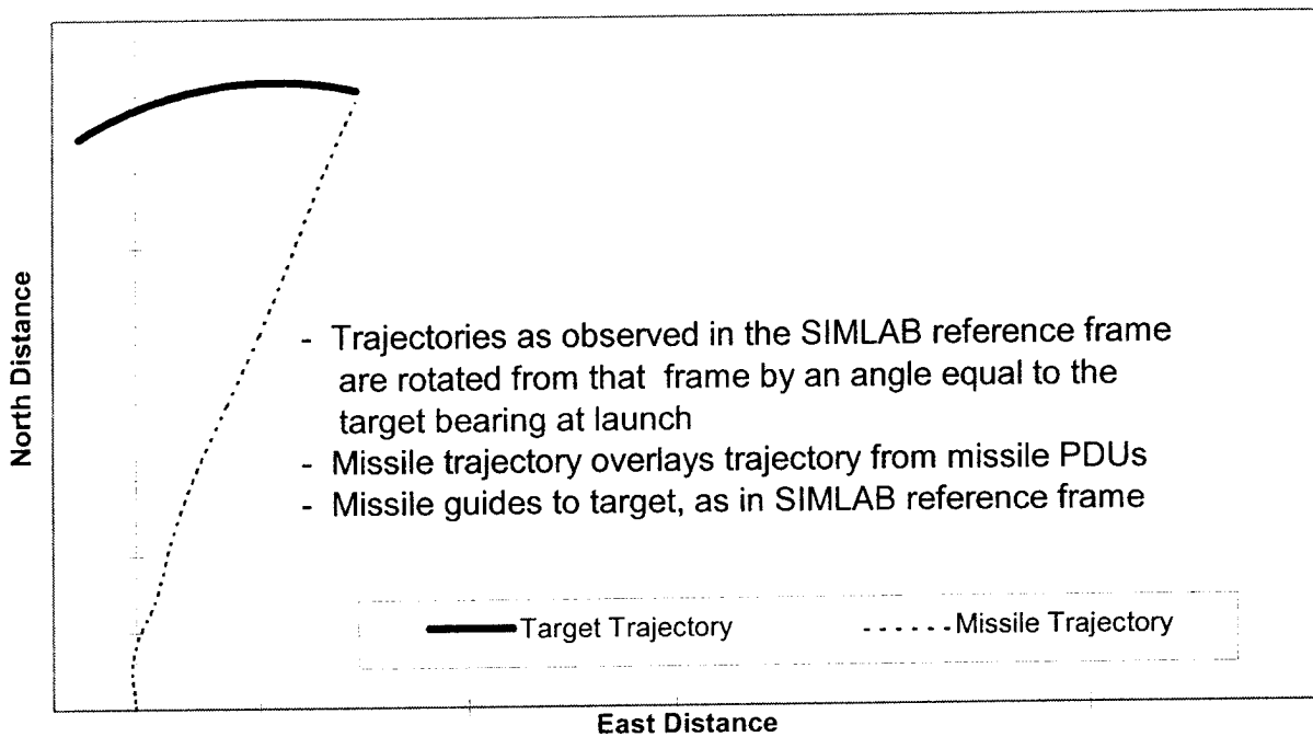
Figure 4.1.1.3-3(a). Missile and Target Trajectories from SIMLAB Data (Run #12 on 11/19/96)
