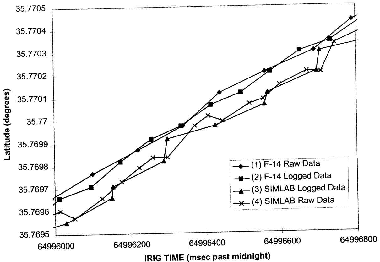
Figure 4.1.1.2-1. Target Latitude vs. Time During Run #23 (10/29/96)
