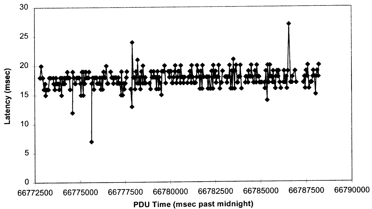
Figure 4.3.3.1-13. Latency of Target Entity State Data (before launch) Between WSIC PDU Logger and WSSF PDU Logger (Run #22 on 11/19/96)
