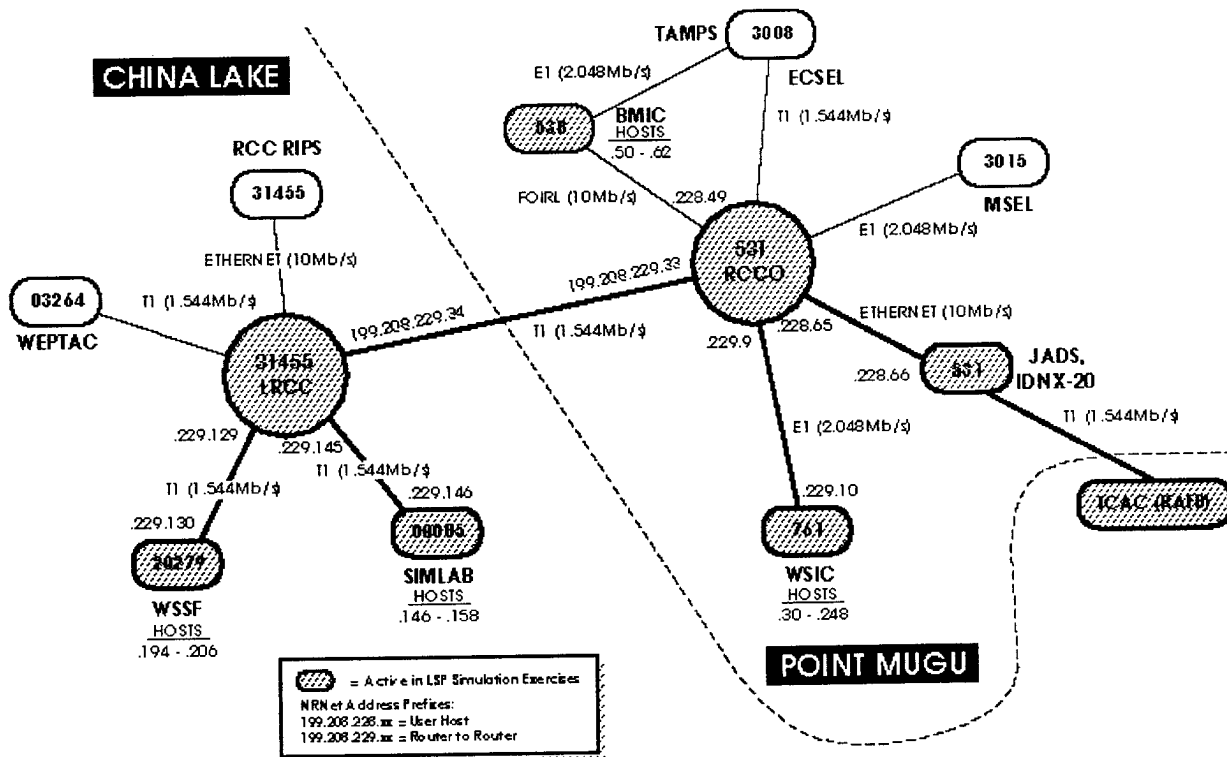
Figure D-2. NRNet Block Diagram
