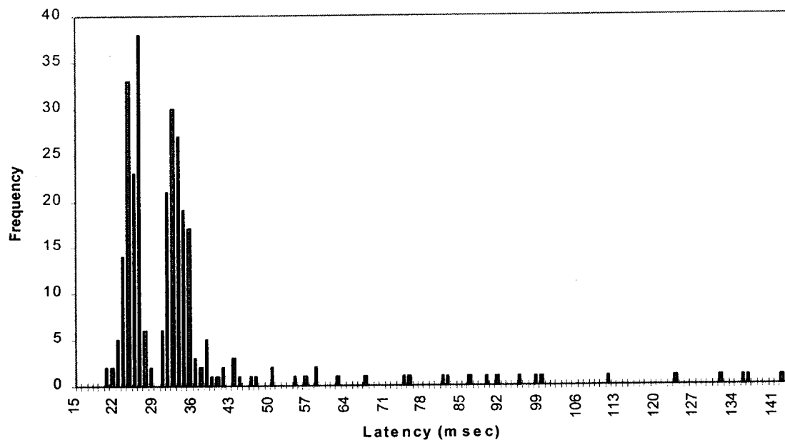
Figure 4.3.3.1-14b. Frequency Histogram of Latency of Target Entity State Data (before launch) Between WSIC Simulation and WSSF PDU Logger (Run #19 on 11/19/96)
