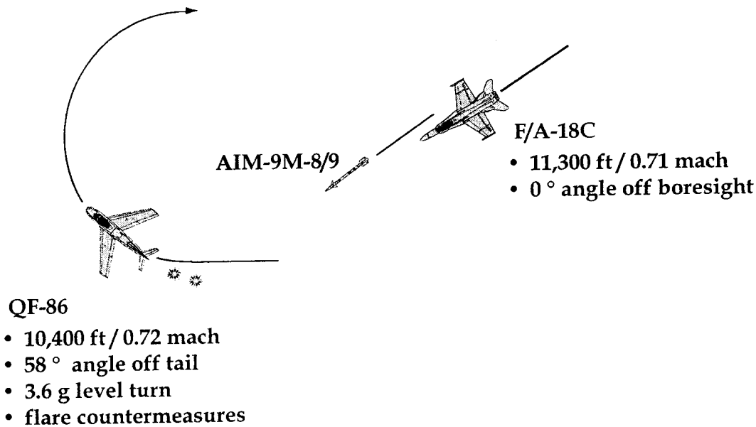
Figure 2.4.1-1. AIM-9M-8/9 Live Fire Profile (LPN-15, 9 June 93)
