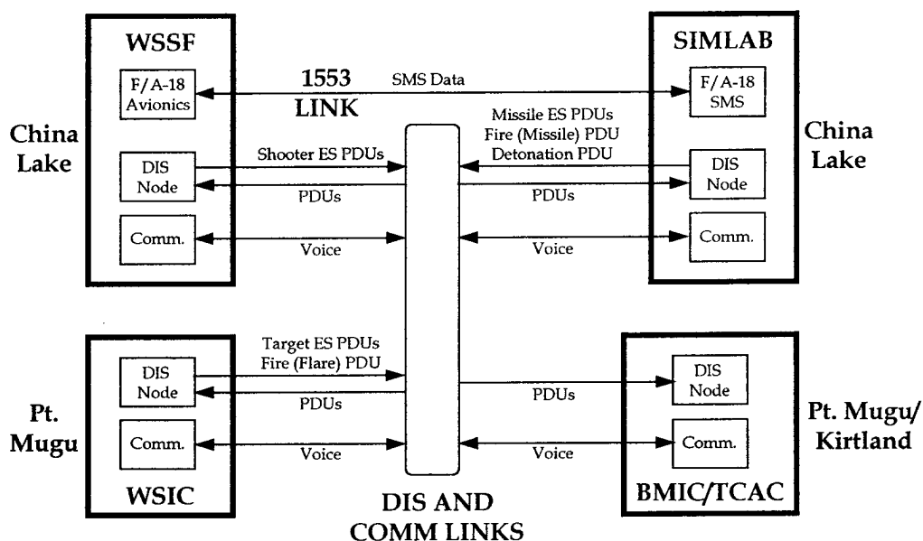
Figure 2.4.3.2-2. Linked Simulators Phase Network Information Diagram
