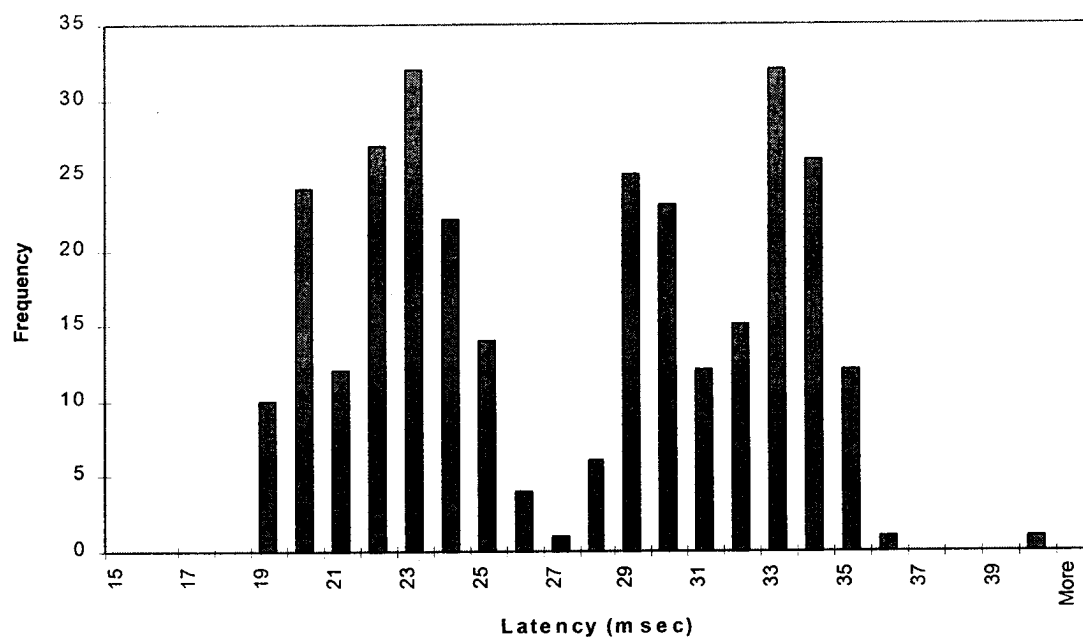
Figure 4.3.3.1-11b. Frequency Histogram of Latency of Target Entity State Data (before launch) Between WSIC Simulation and WSSF PDU Logger (Run #22 on 11/19/96)
