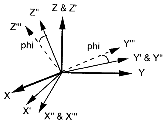
Figure C1-3c. Third Rotate About X\''-Axis By Phi
