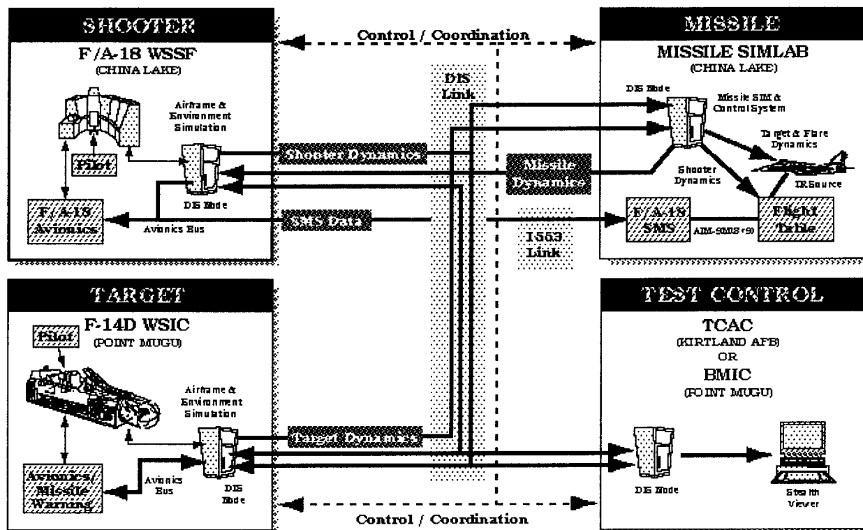
Figure D-1. JADS LSP Configuration
