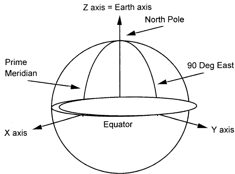
Figure C1-1. World Coordinate System
