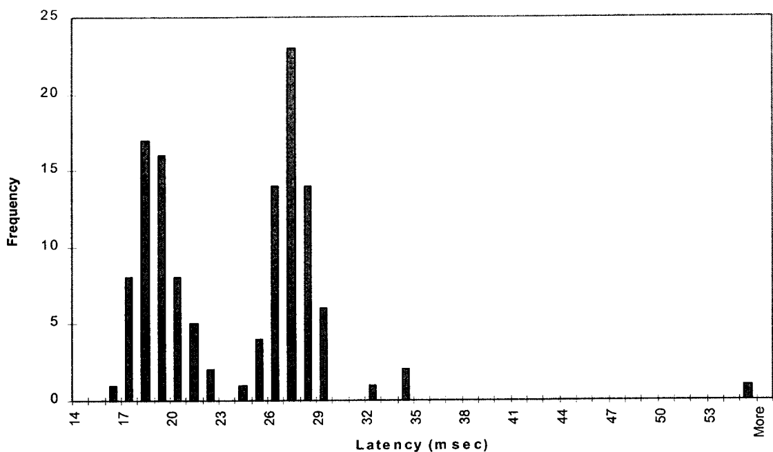
Figure 4.3.3.1-21b. Frequency Histogram of Latency of Target Entity State Data (after launch) Between WSIC Simulation and SIMLAB PDU Logger (Run #9 on 11/19/96)
