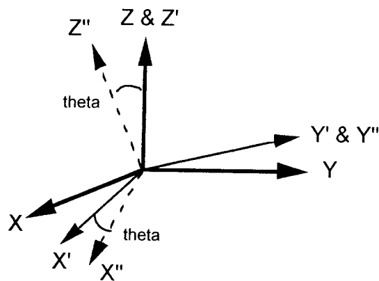
Figure C1-3b. Second Rotate About Y\'-Axis By Theta
