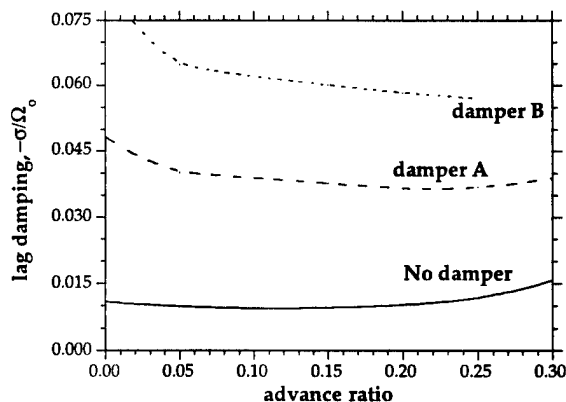
Figure 6: Bearingless rotor shaft-fixed lag stability with inclusion of elastomeric dampers
