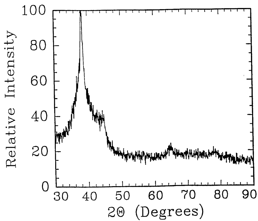
Figure 26. TEM and XRD of Al-5Y-5Fe as-solidified ribbon showing amorphous plus aluminum nanocrystals.
