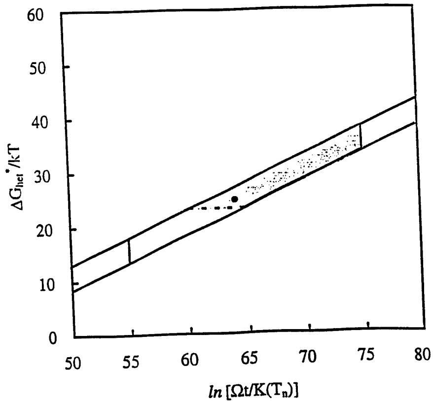
Figure 42. Estimated bounds (solid lines) on \Delta G_{het}^* / kT and \Omega_v t / K(T_n) from kinetics analysis for Al-26 wt % Si alloys.
