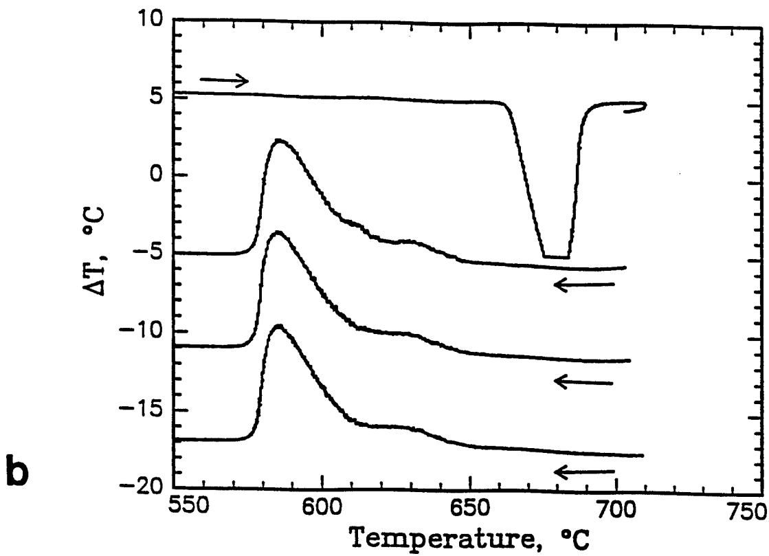
Figure 45. Three consecutive DTA thermograms of 106-125 \mu\text{m} Al-Si 3 N 4 powder (a), and < 53 \mu\text{m} Al-Si 3 N 4 powder (b).
