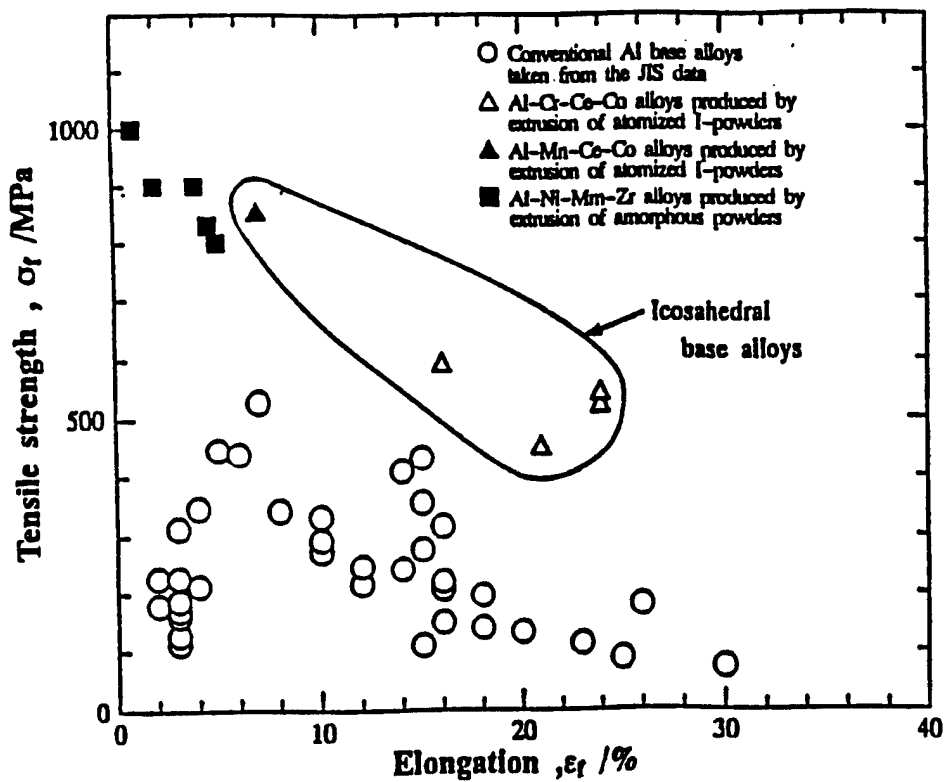
Figure 13. Comparison of \sigma_f and \epsilon_f for icosahedral based alloys and conventional Al alloys [96INO].
