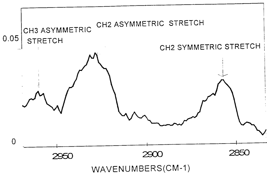
ATR SPECTRA OF 20mM DTAB ADSORBED ON SILICA GEL
