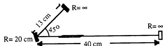
Figure 1. Diagram of laser cavity for TEM 00 mode operation.
