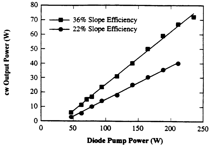
Figure 4. Input vs. output curves for multimode (squares) and TEM 00 mode (circles) operation.
