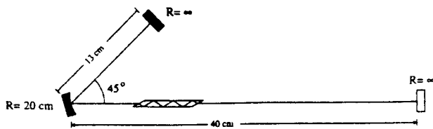
Fig. 2. Cavity design for TEM 00 -mode operation.
