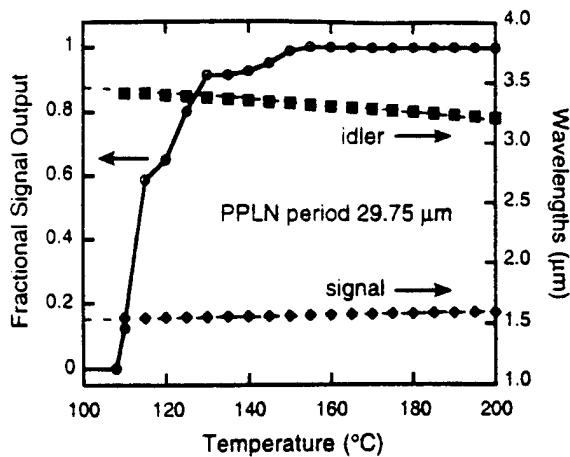
Figure 4. Heating the crystal eliminates photorefractive damage during OPO operation. Temperature tuning is possible as shown, but adjusting the quasi-phasematching period with a multi-grating PPLN chip gave broader tuning over 1.62-1.46 \mu\text{m} (signal) and 3.11-3.95 \mu\text{m} (idler) at 175 ^{\circ}\text{C} for PPLN periods 30-28 \mu\text{m} .
