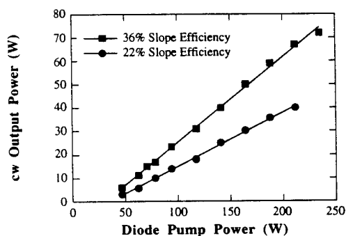
Figure 2. Input vs. output curve for multimode (squares) and TEM 00 mode (circles) operation.
