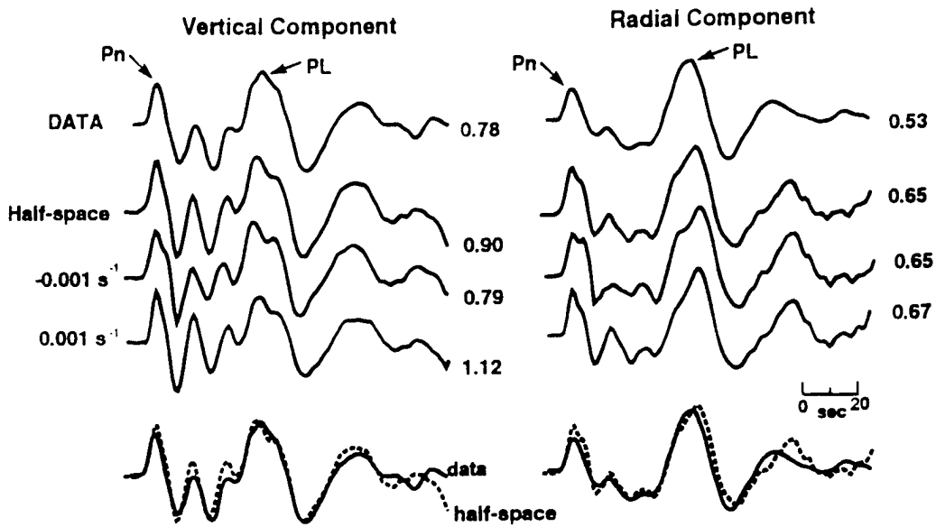
Figure 2: Data and synthetic seismograms for Event 2 (Figure 1) recorded at WIN station. The synthetics are for a halfspace mantle and mantles with P-wave velocity gradients of -0.001 /s and +0.001/s . The numbers to the right of each waveform gives the Pn/PL amplitude ratio. A halfspace mantle works well in explaining these waveforms.
