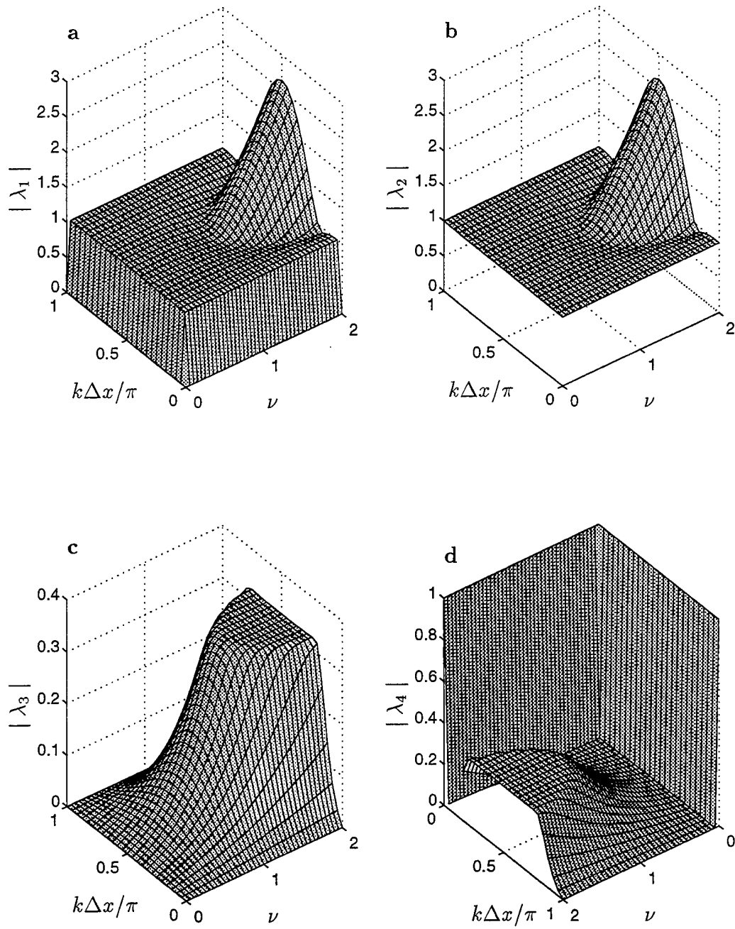
Figure 3.2: Variation of the absolute eigenvalues |\lambda_p| versus the Courant number \nu and the wave number k\Delta x : (a) |\lambda_1| ; (b) |\lambda_2| ; (c) |\lambda_3| ; (d) |\lambda_4| .
