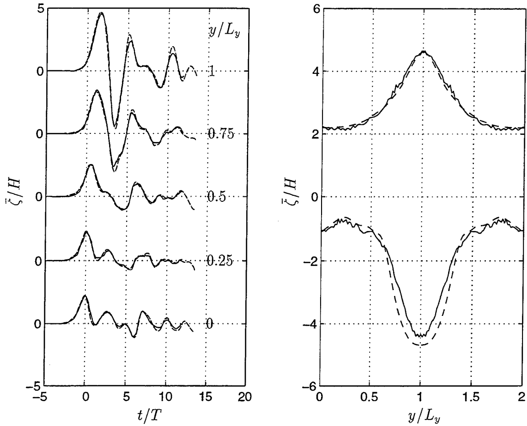
Figure 3.19: Comparison of present model (—) to Zelt (1986) (---) for \alpha = 0.02 : (a) Timeseries of run-up in 5 stations, (b) Maximum run-up and run-down.
