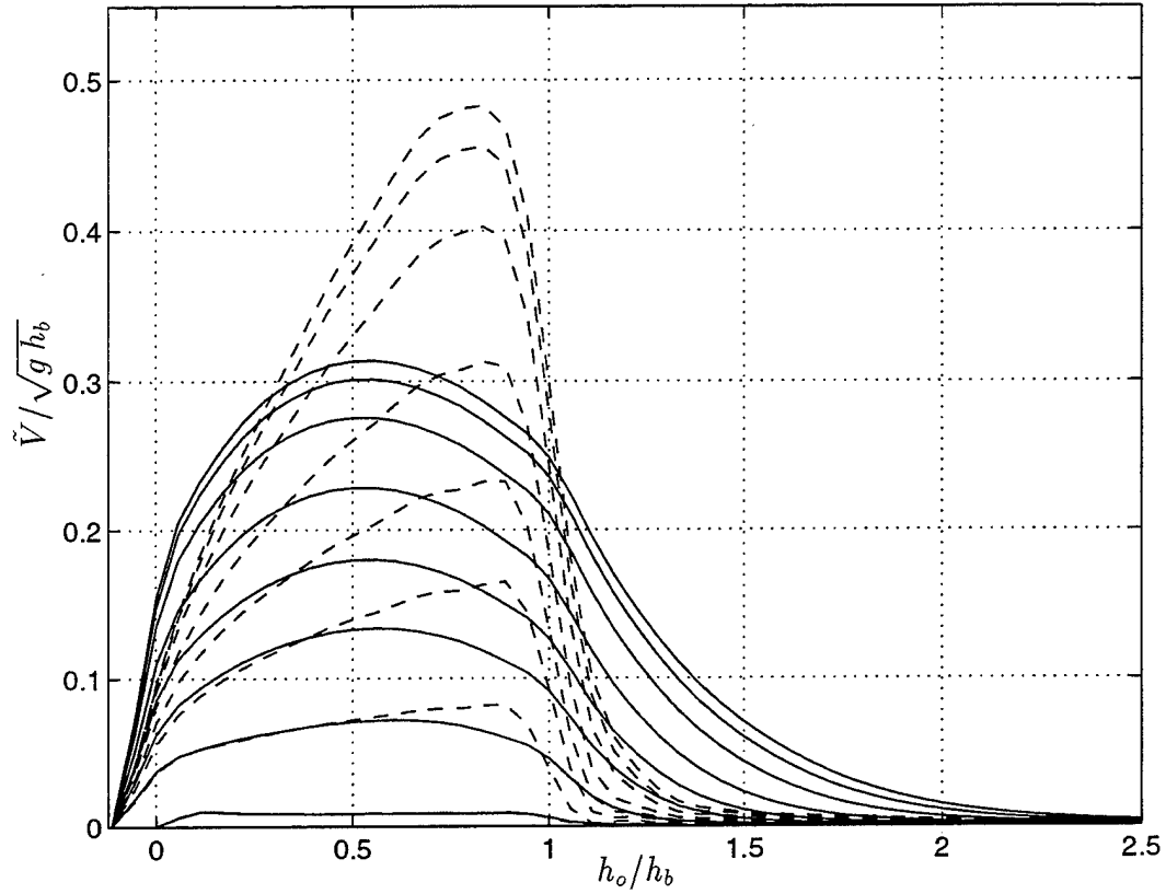
Figure 5.2: Normalized longshore current velocities versus normalized depth with quasi 3-D terms (—) and without quasi 3-D terms (— —) at t = 0, 2, 6, 10, 14, 20, 30, 40 and 48 T .
