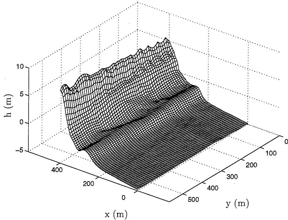
Figure 3.1: Typical bathymetry at the U.S. Corps of Engineers' Field Research Facility at Duck, NC taken on October 10, 1990.
