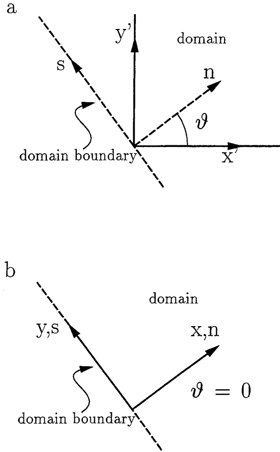
Figure 3.5: Coordinate system (a) for arbitrary angle \vartheta between domain boundary and x -axis; (b) for \vartheta = 0 .
