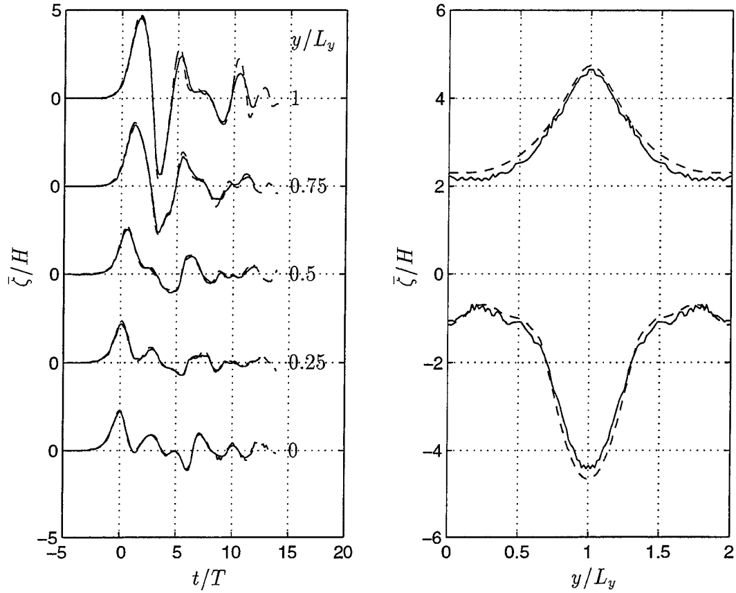
Figure 3.20: Comparison of present model (—) to Özkan-Haller & Kirby (1997) (---) for \alpha = 0.02 : (a) Timeseries of run-up in five stations, (b) Maximum run-up and run-down.
