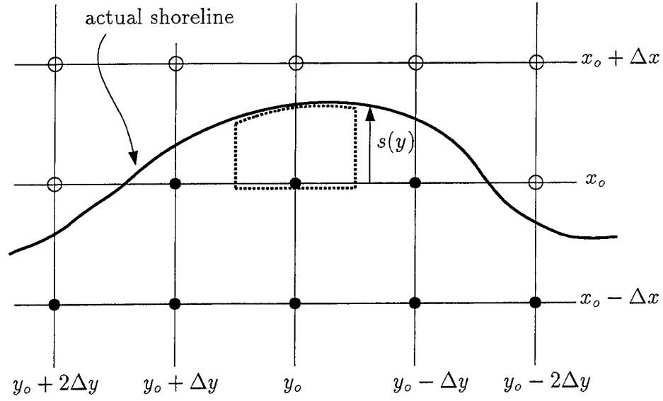
Figure 3.15: Plan view of an arbitrary shoreline on a fixed grid with inundated nodes (•) and “dry” nodes (o).
