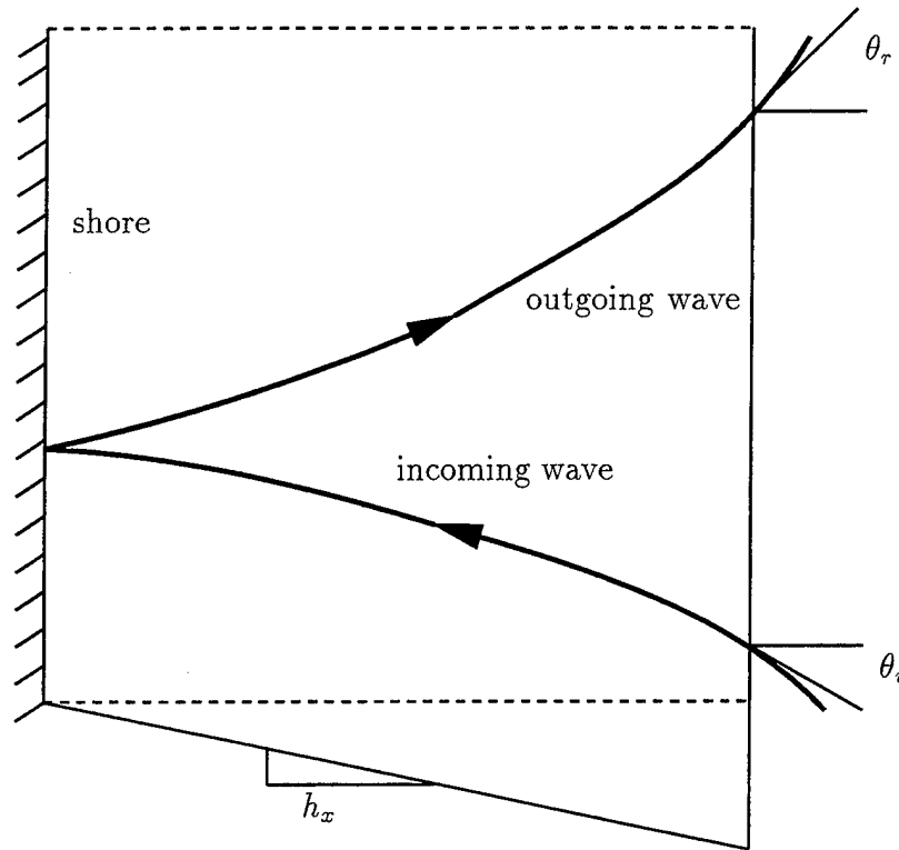
Figure 5.7: Definition sketch of obliquely-incident and obliquely-reflected infragravity waves.
