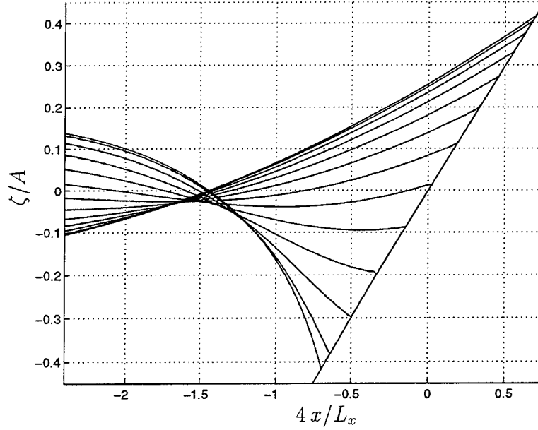
Figure 3.16: Comparison of present model (—) to Carrier & Greenspan (---) for A = 0.7 for time-instances at intervals of 0.13 T
