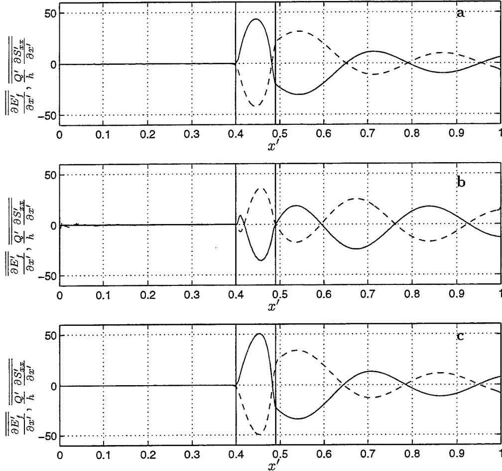
Figure 4.21: Work done on total long wave (—) and energy flux (---): (a) Nonlinear version; (b) Linear version; (c) Linear version with mean set-up included in the depth.
