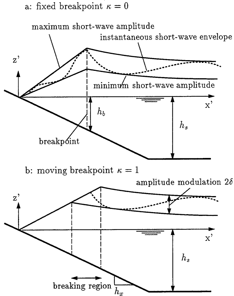
Figure 4.1: Definition sketch of the generation mechanisms: a) Schäffer & Svendsen (1988)'s fixed breakpoint generation mechanism. b) Symonds et al. (1982)'s moving breakpoint generation mechanism. (Reproduced from Schäffer, 1993)
