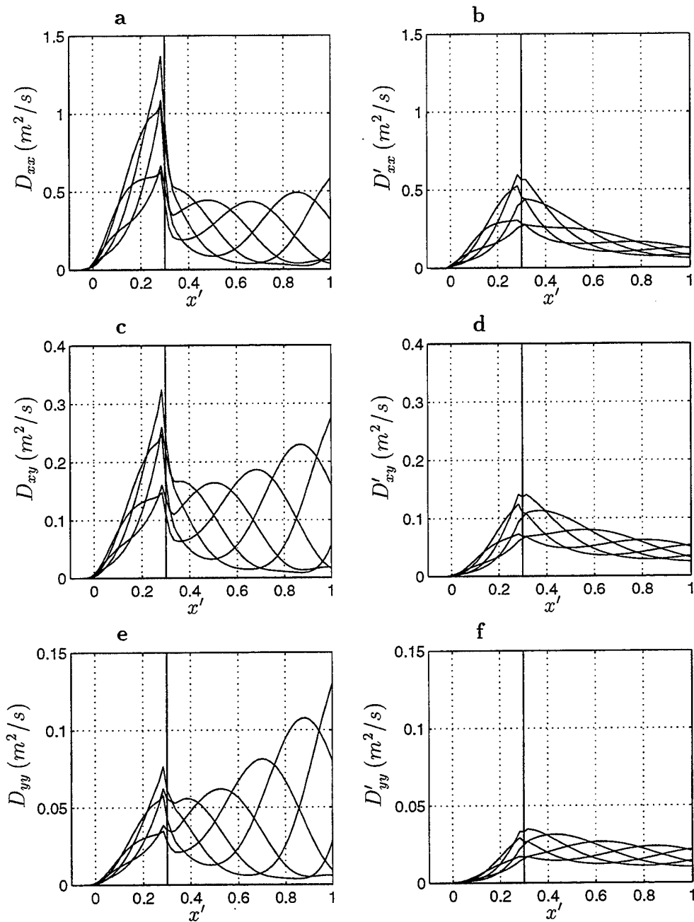
Figure 5.15: Comparison of D coefficients for five intervals per IG wave period: (a) D_{xx} . (b) D'_{xx} = \frac{Q_{wx}^2}{3\nu_t} . (c) D_{xy} . (d) D'_{xy} = \frac{Q_{wx}Q_{wy}}{3\nu_t} . (e) D_{yy} . (f) D'_{yy} = \frac{Q_{wy}^2}{3\nu_t} .
