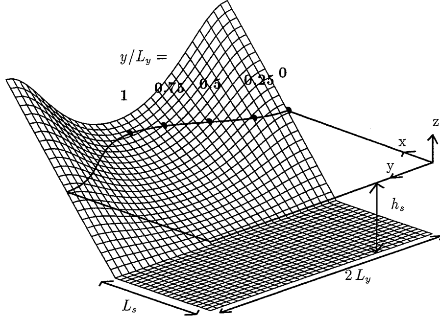
Figure 3.18: Definition sketch of the concave beach bathymetry (courtesy Dr. H.T. Özkan-Haller)
