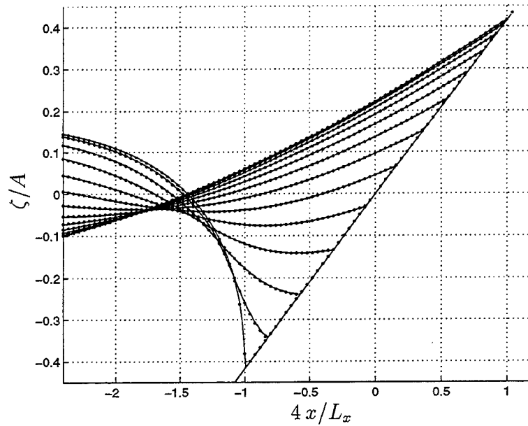
Figure 3.17: Comparison of present model (—) to Carrier & Greenspan (•••) for A = 1.0 for time-instances at intervals of 0.13 T
