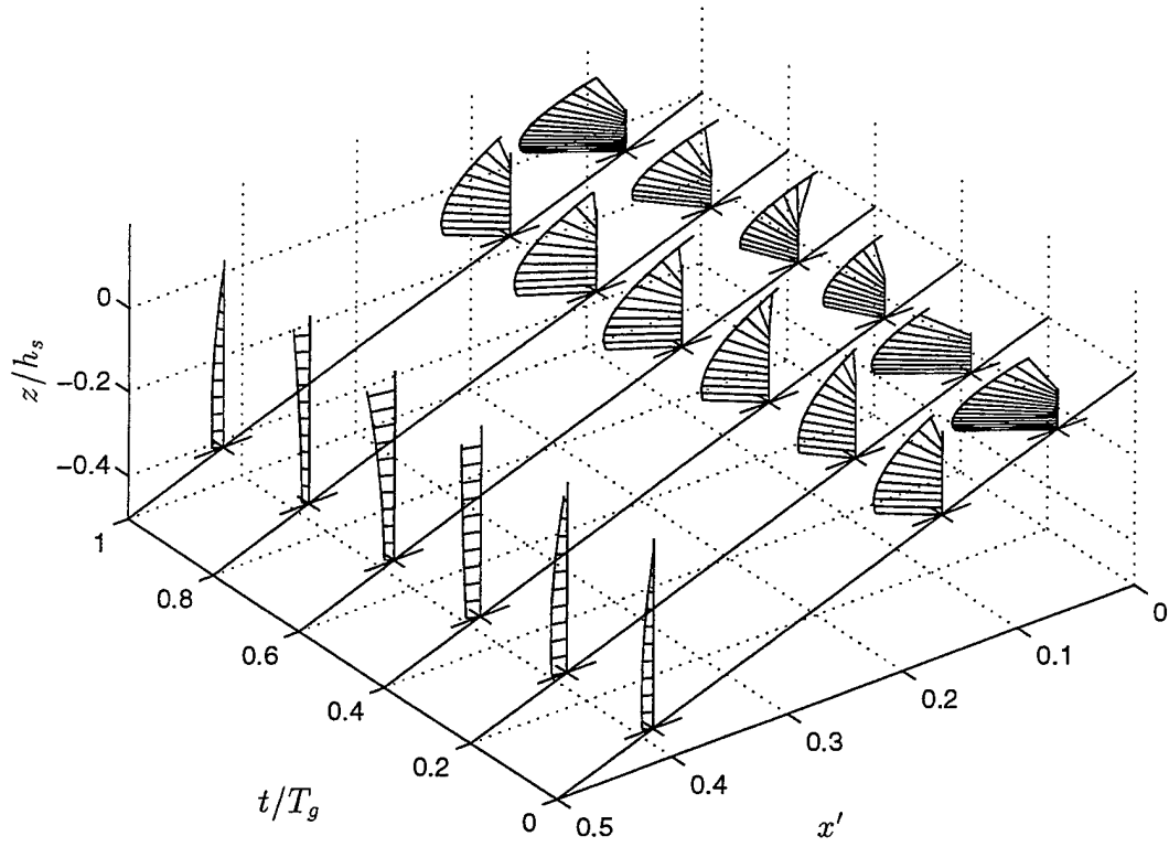
Figure 5.12: Infragravity wave profiles for three locations ( x' = 0.42, 0.17 and 0.07 ) and for five time instances of the infragravity wave period. The breakpoint is located at x' = 0.3 .
