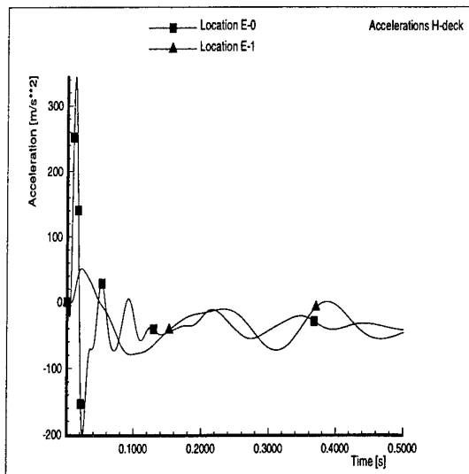
a) Location E-0, E-1, large time period (close to location E (midway hull and corrugated plate), but at discrete mass) b) Location E-0, short time period
