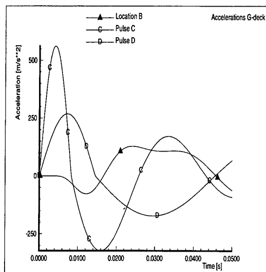
h) Accelerations location B (centre of compartment)
