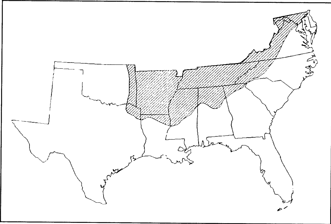
Figure 1. Potential breeding distribution of the cerulean warbler in the southeastern United States (from Robbins et al. 1992, Hamel 1992b)
