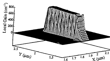
4. Simulated gain profile for an LCI laser with current guiding layers [6]. A 0.1- \mu\text{m} thick active region extends from the n-type regrowth at Y = 1.5 \mu\text{m} to the p-type regrowth at Y = 2.5 \mu\text{m} . The region above the active layer ( X < 1.8 \mu\text{m} ) is p-type and the region below ( X > 1.9 \mu\text{m} ) is n-type.
