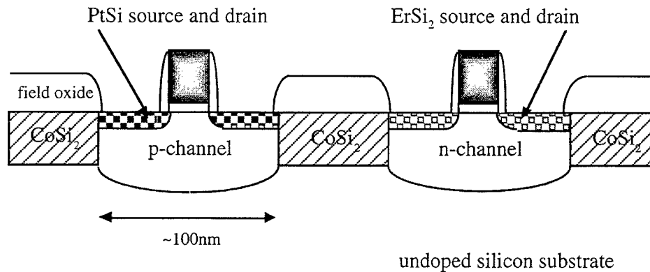
Fig. 3 Sketch of future ~25nm gate-length Schottky barrier CMOS inverter with buried, epitaxial, and self-planarized \text{CoSi}_2 local interconnects.
