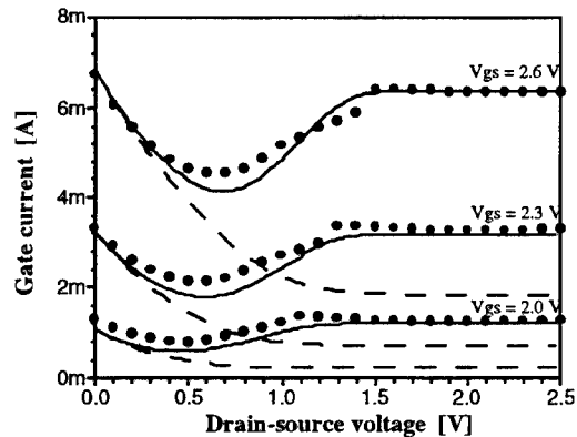
Fig. 4a. Measured (symbols) and simulated gate current versus V_{ds} for a 0.8\ \mu\text{m} long, 10\ \mu\text{m} wide HFET. Dashed lines corresponds to simulation results with the hot-carrier effect disabled in the model. Data from Lee et al. [8].
