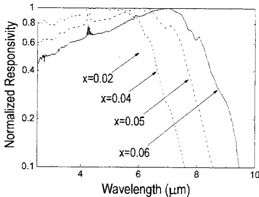
Figure 9. The normalized spectral response of the \text{In}_{1-x}\text{Ti}_x\text{Sb} photoconductors at 77 K.
