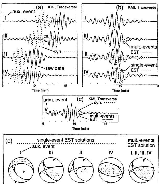
Figure 7. (a) Transverse-component displacement waveforms (solid lines) recorded at station KMI ( 25^\circ in distance and 103^\circ in azimuth from the 18 March 1995 earthquake) from various auxiliary events along with synthetics (dashed lines) computed using the Harvard CMT solutions for events I, II, and III and the EST solution for event IV. (b) Solid lines show the multiple-events EST waveform obtained using \alpha that is calculated by interpolating observed \alpha for various auxiliary events; dashed lines show single-event EST waveforms obtained using observed \alpha for each auxiliary event. (c) The multiple-events EST waveform (solid line) and synthetic waveform (dashed line) computed using the solution obtained from inversion of multiple-events EST waveforms. (d) Focal mechanism solutions obtained from inversions of single-event EST waveforms for each auxiliary event and from inversion of multiple-events EST waveforms.
