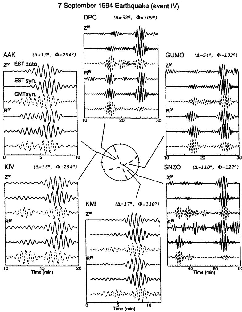
Figure 4. Vertical ( Z^{IV} ) and radial ( R^{IV} ) components of EST waveforms (thin solid lines) and synthetics for the 7 September 1994 earthquake. Thick solid lines show synthetics computed using the EST solution obtained in this study, which has a depth of 13 km. Dashed lines show synthetics computed using the Harvard CMT solution, which has a depth of 33 km. Nodal lines on the focal sphere are for the EST solution.
