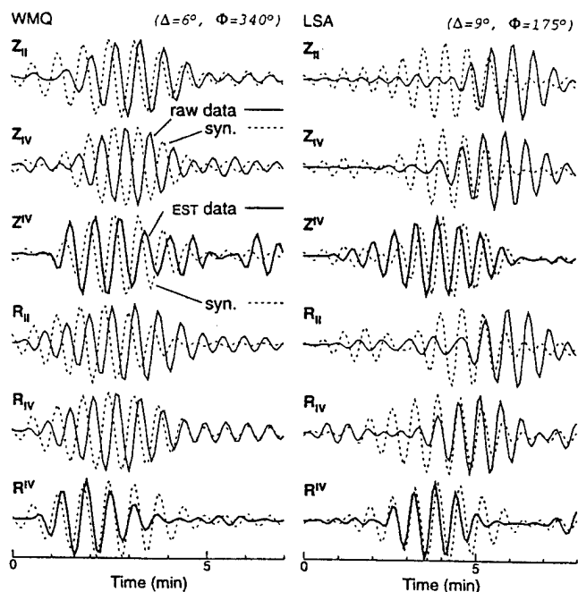
Figure 5. Vertical ( Z ) and radial ( R ) components of displacement waveform data (thin solid lines) for two stations at regional distances from the 7 September 1994 (event IV) and the 2 October 1993 (event II) earthquakes (subscript identifies the event). EST waveforms (thick solid lines) are shown for event IV ( Z^V and R^V ). Synthetics (dashed lines) are computed for event II (auxiliary event) using the Harvard CMT solution and for event IV (primary event) using the EST solution obtained in this study.
