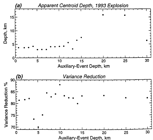
Figure 9. (a) Apparent depth of the centroid of the 5 October 1993 explosion plus tectonic release obtained from inversions of EST waveforms, which are calculated using the 21 May 1992 explosion as the auxiliary event. Abscissas indicate assumed centroid depths of the auxiliary event in calculation of EST waveforms. (b) Maximum variance reduction in iterative inversions of EST waveforms.
