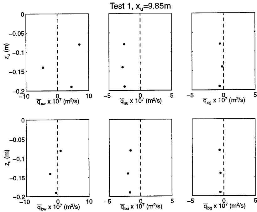
Figure 6.7: Variation of Suspended Load and Bed Load Quantities Over Depth at x = 9.85 \text{ m} , Test 1 (Energetics Model)
