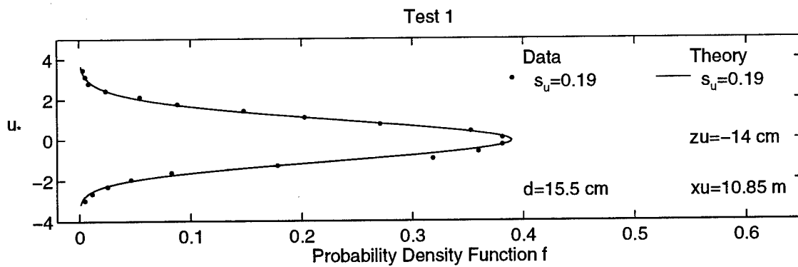
Figure 5.16: Measured and Computed Probability Distributions for Horizontal Velocity at Position x = 10.85 \text{ m} for Test 1
