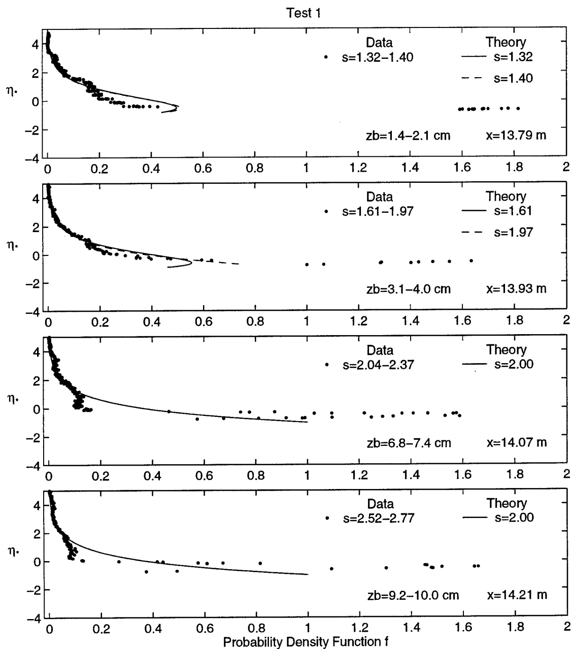
Figure 4.23: Measured and Computed Probability Distributions at Positions x = 13.79, 13.93, 14.07 , and 14.21 m for Test 1
