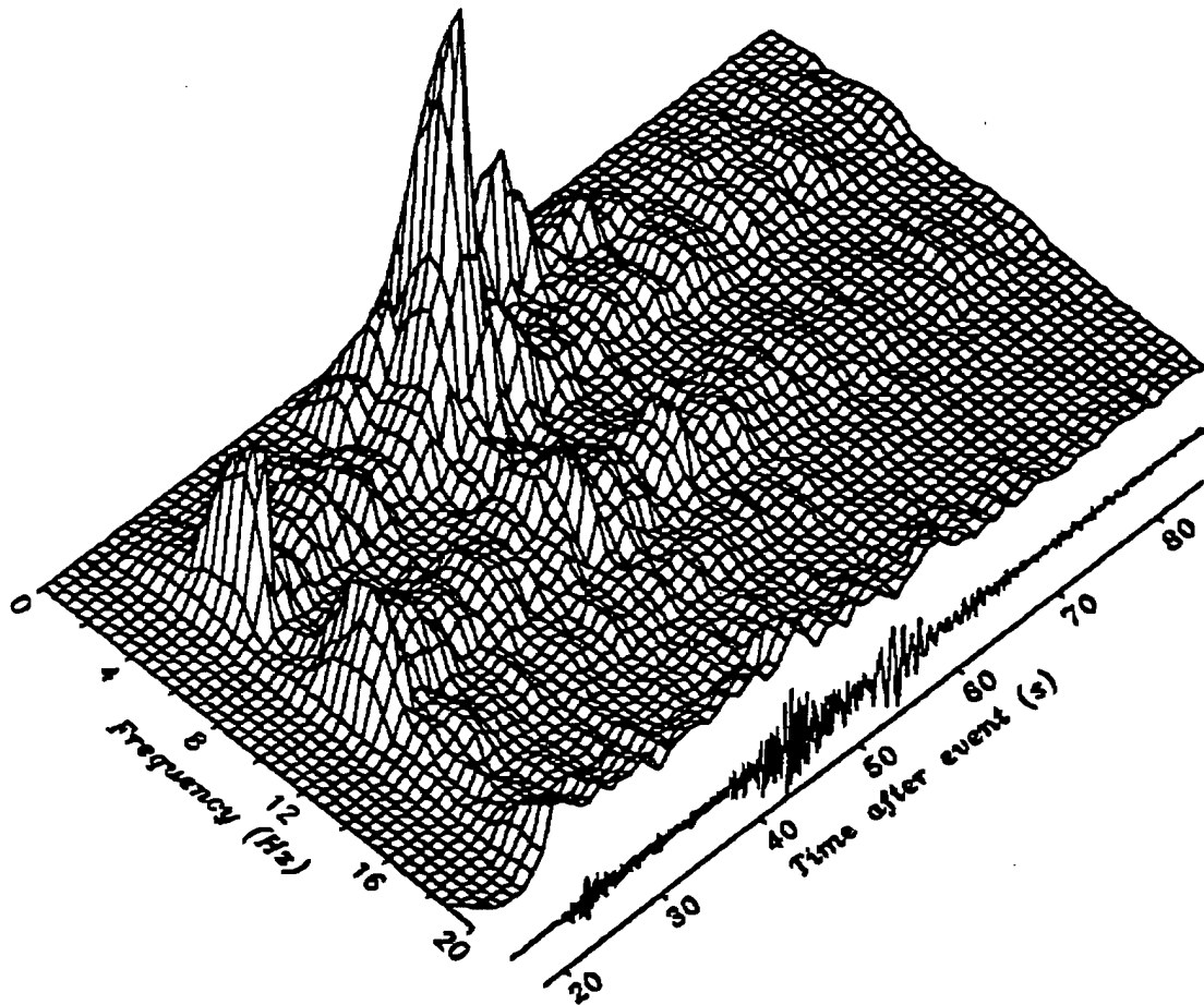
Figure 2.5 Spectrum from synthetic consisting of 39 cospatial shots spaced at regular time intervals of 25 ms; the Green's function for this synthetic is the single calibration explosion Chemex 2 examined in this paper. Credit: Hedlin, 1991.
