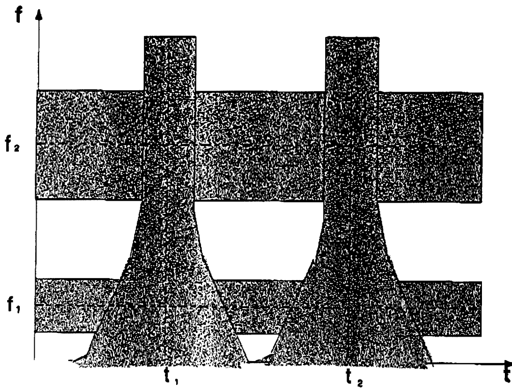
Figure 2.9 Fourier and wavelet decompositions are applied to the function \delta(t - t_1) + \delta(t - t_2) + \exp(i2\pi f_1 t) + \exp(i2\pi f_2 t) , which in effect images the resolving power of the transform in both the time and frequency domains; the Fourier spectrum is pictured above,
