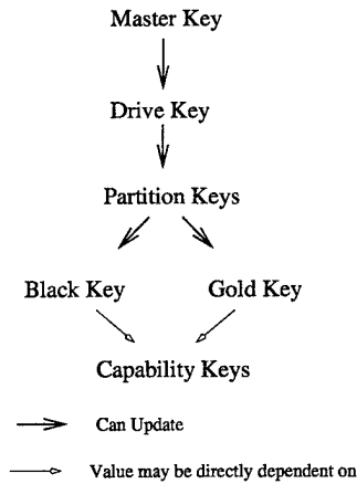
Figure 3: Key Hierarchy Relationships
