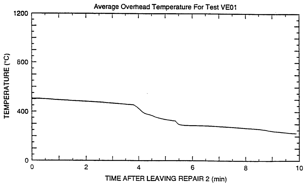
Fig. A1 — Wood crib and average overhead temperatures for test VE01
