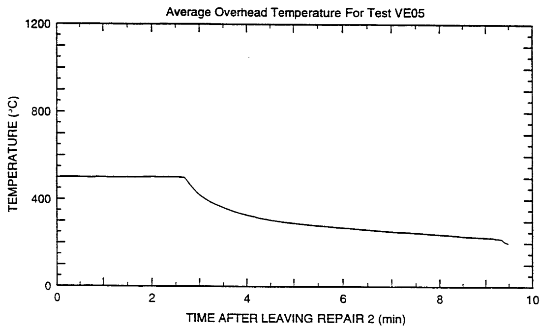
Fig. A9 — Wood crib and average overhead temperatures for test VE05
