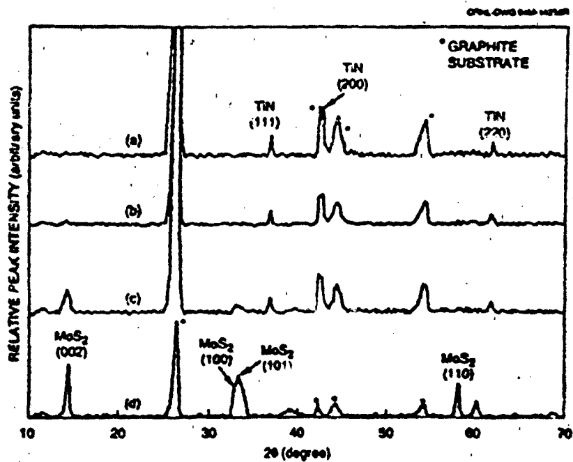
Fig. 1. XRD patterns of multiphase coatings deposited at 820°C and inlet MoF 6 partial pressures of: (a) 2.8 Pa, (b) 6.9 Pa, (c) 9.6 Pa, and (d) 13.6 Pa. All other process parameters were kept constant for the deposition experiments. From Ref. (15).
