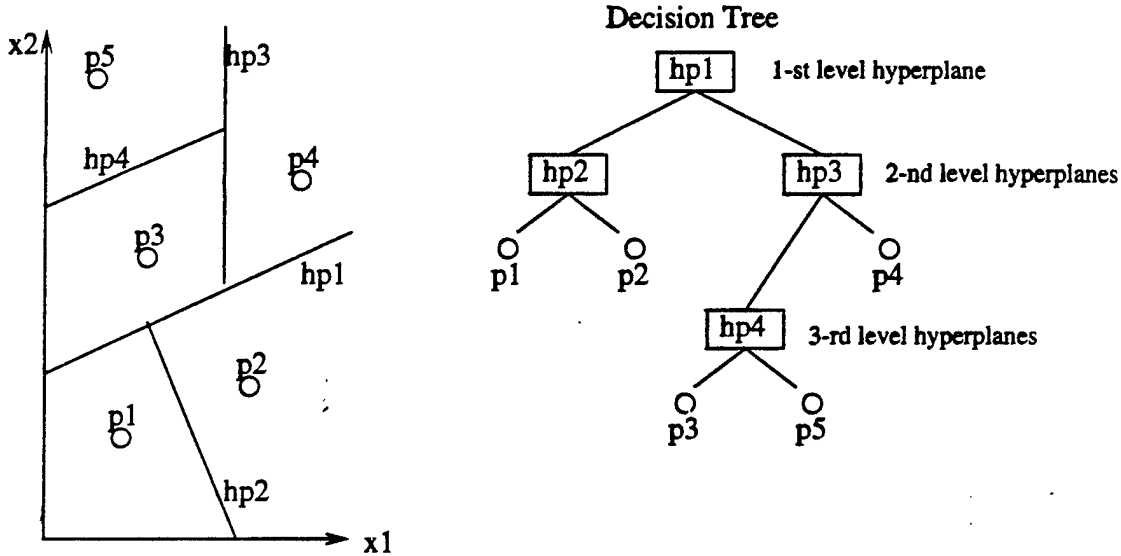
Figure 8: Decision Tree Construction
