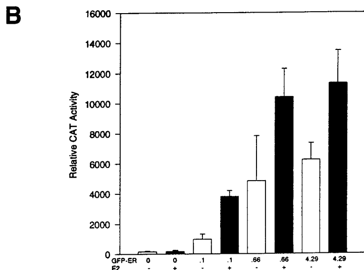
Figure 4. Ligand Regulation of the pERE-tk-CAT reporter vector by GFP-ER in MDA MB 435A cells. Panel A. Lane 1 - no ligand added. Lane 2 - 0.1nM 17 \beta -estradiol. Lane 3 - 1nM 17 \beta -estradiol. Lane 4 - 10nM 17 \beta -estradiol. Lane 5 - 100nM 17 \beta -estradiol. Lane 6 - 10nM ICI 182 780. Lane 7 - 10nM 4-hydroxytamoxifen. Lane 8 - 500nM ICI 182 780 and 10nM 17 \beta -estradiol. Lane 9 - 250nM 4-hydroxytamoxifen and 10nM 17 \beta -estradiol. (All transfections in Panel A are with 0.1 \mu g of pCI-nGFP-ER). Panel B. White bars represent no ligand added, black bars represent 10nM 17 \beta -estradiol added. Increasing amounts of GFP-ER expression plasmid ( \mu g) were transfected. All experiments done in triplicate.
