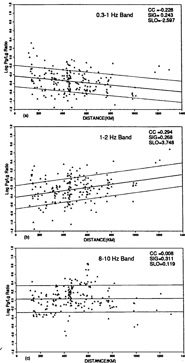
Figure 2. \log(P_g/L_g) as a function of distance in various frequency bands: (a) 0.3 to 1.0 Hz, (b) 1.0 to 2.0 Hz, (c) 8.0 to 10.0 Hz. CC indicates the correlation coefficient, SIG is the standard deviation of the regression, and SLO is the slope of the regression line.
