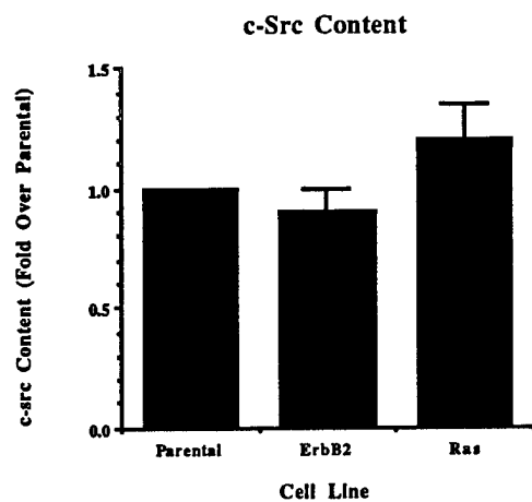
Figure 10. Effect of ErbB2 or ras transformation of 184.A1 cells on c-src content, as determined by Western blot analysis. Mean ± SEM of 4 determinations.
