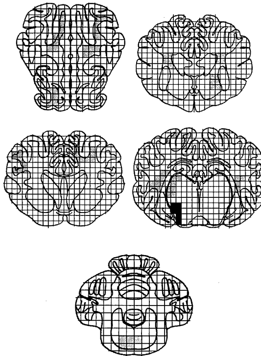
Figure 6 - Injury patterns in the miniature pig brain were in multi-focal regions throughout the white matter. Shown are the injured regions across five coronal sections in a miniature pig experiment (Scale: cross-hatch = 1-5 injured axons/field; gray = 6-15 injured axons/field; black = >15 injured axons/field).
