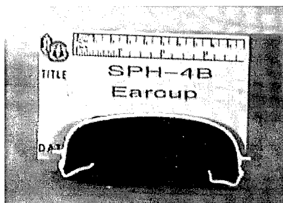
Figure 12. SPH-4B earcup, cross section.
