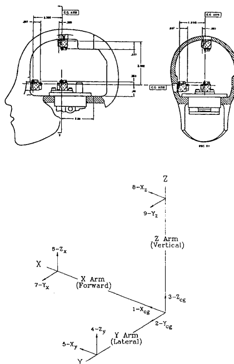
Figure 1: (a) Accelerometer Locations in Dummy Headpart 3-2-2 Arrangement (b) Ideal 3-2-2 Configuration
