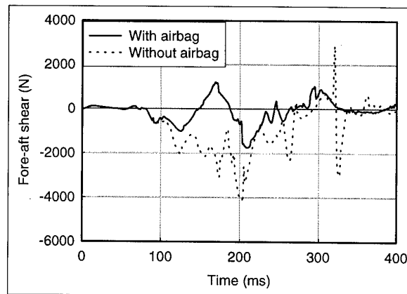
Figure 8 - Fore-aft shear force at the head-neck joint for simulations where the harness worked properly.
