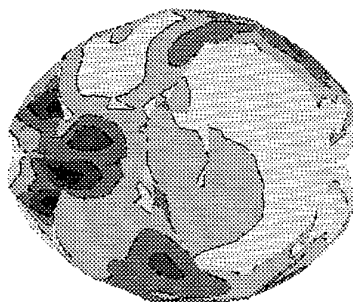
Figure 16 Shear stress contours - bottom view.
