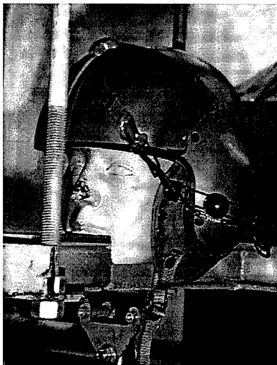
Figure 15. Chin strap static pull test setup.
