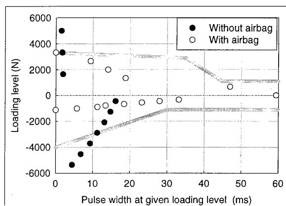
Figure 12 - Injury assessment of neck axial force for simulated malfunctioned harness.
