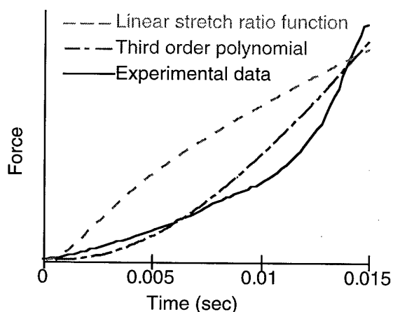
Figure 11: Model simulations of dynamic optic nerve elongation using a linear and a third-order polynomial elastic function along with experimental data. The third order polynomial model better predicted the experimental data.
