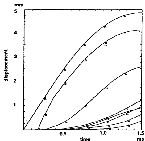
Figure 5 The results from Dyna3d: The resultant total displacement history of the selected nodes, 10011 (A, impactor), 3982(B, brain impact surface), 4017(C), 4074(D), 4089(E), 4086(F, contra-lateral brain site), 4125(G, brain bottom surface) and 6354(H, spinal cut ending) are shown. There is a gap (0.8 mm) between the impactor tip and the brain impact surface.
