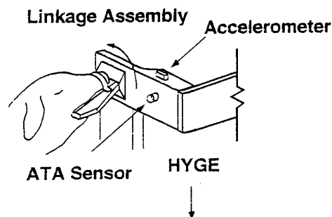
Figure 2 - Schematic of experimental model of diffuse axonal injury in the miniature pig. The animal's head is secured in a head holder apparatus and accelerated through an angle of either 94 or 104 degrees, depending upon the linkage design. Acceleration is restricted to the coronal plane since this is the plane often associated with DAI.
