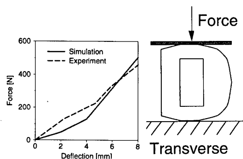
Figure 2 Force deflection curve of outer shell only, in transverse loading direction, and test setup used.
