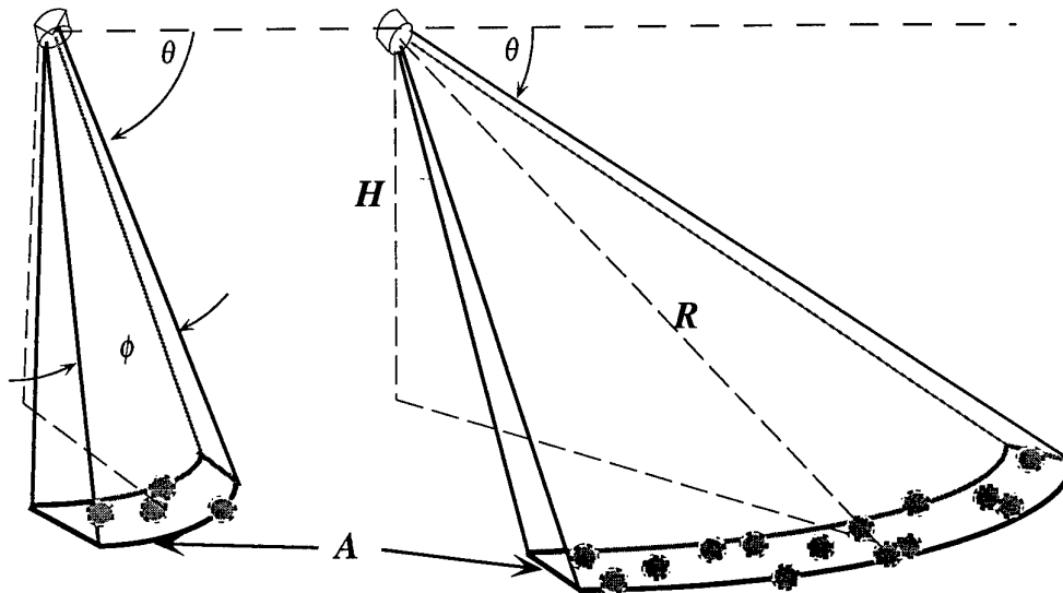
Figure 2 Experimental configuration.
