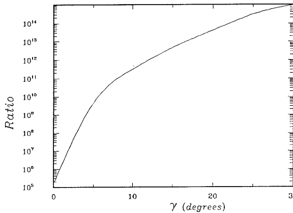
Fig.2 Comparison of the indirect transition via the gamma-deformed state and the direct case. The figure gives the ratio of T(EM, 16_7^+ \rightarrow 12^-(K=8)) over T(E9/M8, 16^+(K=16) \rightarrow 14^-(K=16)) . Our calculation is based on the single-particle Weisskopf units and the energy spacings are assumed to be 1 MeV.
