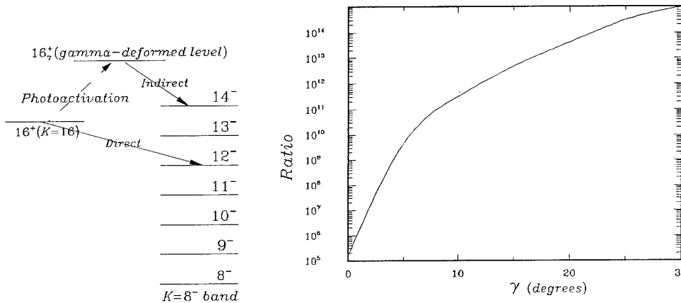
Fig.1 Modeled nuclear levels and two EM transition schemes for depopulating the isomer 16^+(K=16) .
