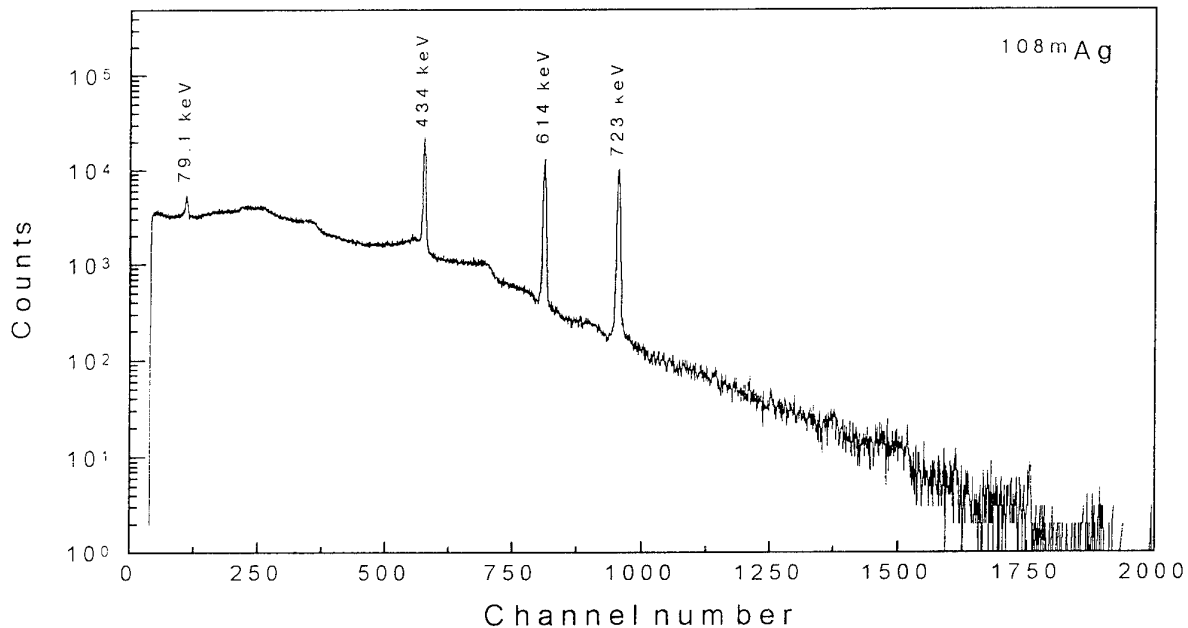
Fig. Spectrum of ^{108m}\text{Ag} \gamma -rays following neutron excitation of ^{\text{nat}}\text{Ag} . Cooling time is more than 13 years. Number of nuclei in the ^{108m}\text{Ag} isomeric state with J^\pi = 6^+ is 10^{17} .
