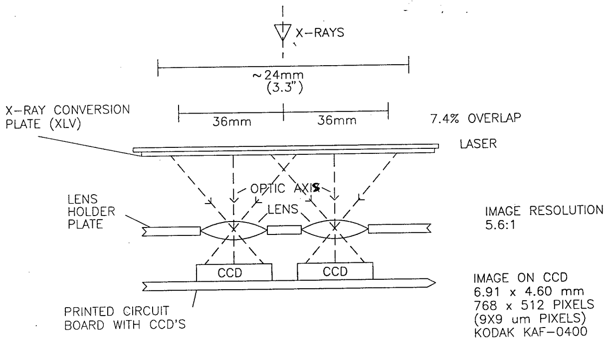
Fig. 6 Optics for One Segment
