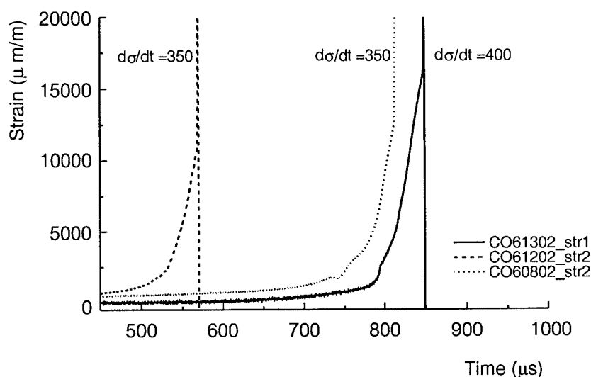
Figure 4: HTPB and PPG strain results with a derivative of 350 and 400 \text{m}/\text{m}\cdot\text{s} .
