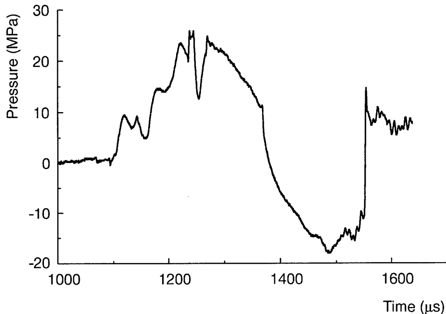
Figure 6: A pressure measurement of a HTPB/AP Cook-off experiment.
