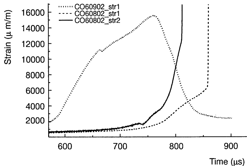
Figure 2: Strain gauge results of PPG/APIAN Cook-off experiments.
