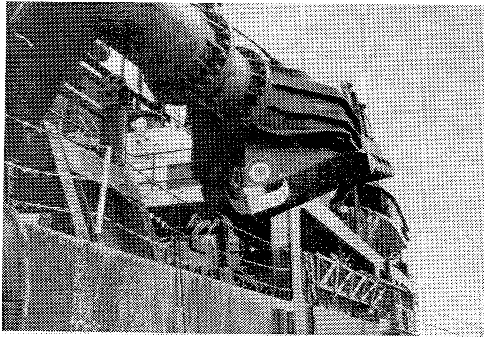
Figure 3. Prototype rigid deflector draghead installed on McFarland's port dragarm (after Banks and Alexander (1994))
