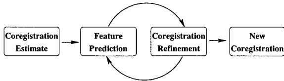
Figure 8: Interleaving Feature Prediction, Coregistration Refinement and Matching
