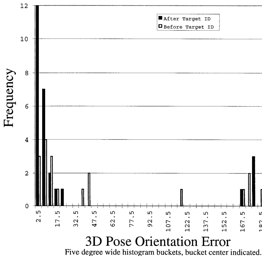
Figure 13: Difference between estimated and true 3-D target orientation before and after running of the multisensor identification algorithm. Bars labeled 'Before Target ID' indicate pose estimates coming out of the hypothesis generation algorithm, and those labeled 'After Target ID' are after multisensor matching has been run. Frequency is the count of trials with pose estimates differing from ground truth by the indicated amount.
