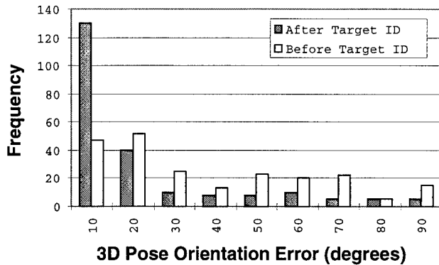
Figure 14: Difference between estimated and true 3-D target orientation before and after running of the multisensor identification algorithm.
