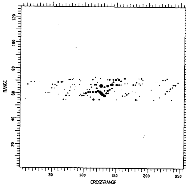
Figure 59. Image of M-60 Moving in a Circle, Aspect Angle of 30^\circ .
