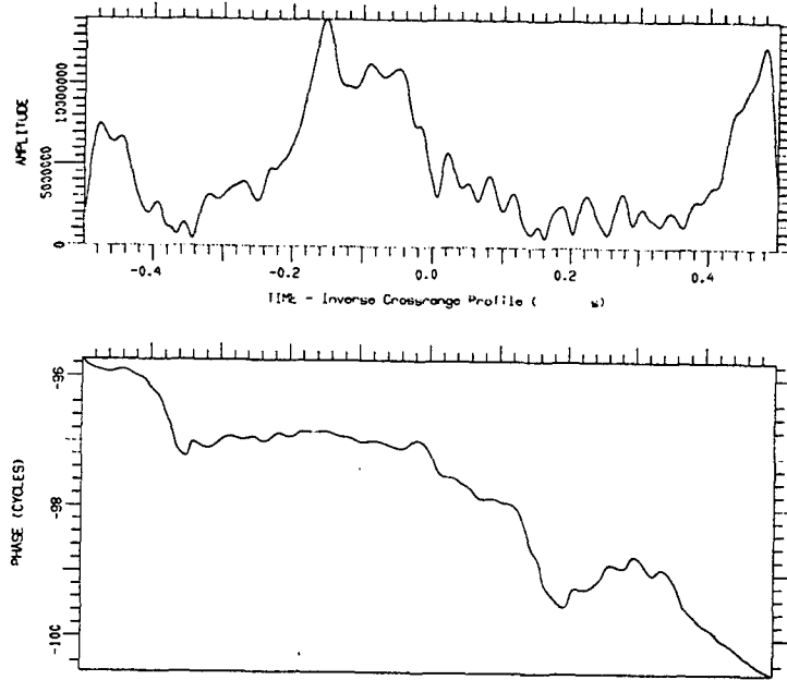
Figure 43. Transform of Image Cut in Range Gate 41.83.
