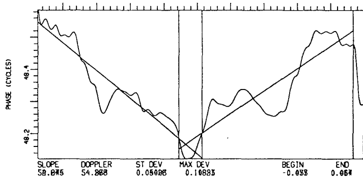
Figure 15. Transform of Image Cut in Range Gate 26.80.
