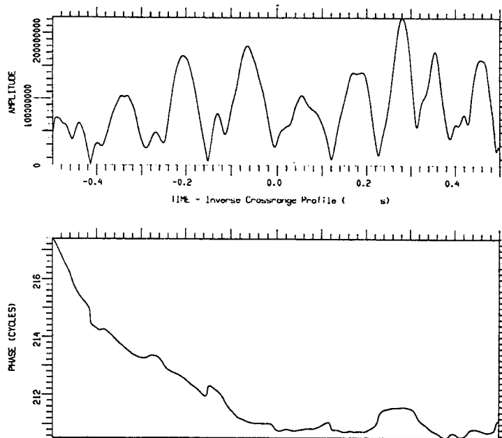
Figure 2. Image Cut in Range Gate 55.69.
