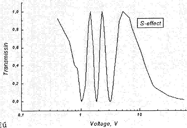
Fig. 3. Electro-optical characteristic of the SLM on optical birefringence, thickness of LC layer is 20 \mu\text{m} .
