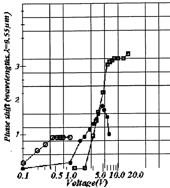
Fig.3.2. Experimentally measured phase shift on double pass through the SLM vs. applied voltage; \Delta n \approx 0,16 ; rings correspond to LC thickness of 5 \mu\text{m} (two specimens with different properties of ZnSE layer), empty squares correspond to the LC thickness of 10 \mu\text{m} .
