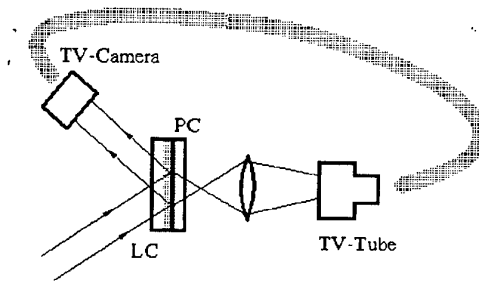
Fig.6.8. Feedback lock by the system: TV-camera-TV-tube-projectile optics-OA SLM
