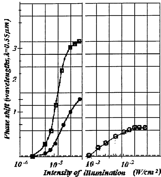
Fig.3.3. Experimentally measured phase shift on double pass through the SLM vs. intensity of controlling radiation; \Delta n \approx 0,16 ; rings correspond to LC thickness of 5 \mu\text{m} (two specimens with different sensitivity of ZnSE layer), empty squares correspond to the LC thickness of 10 \mu\text{m} .
