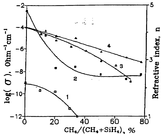
Fig.21. Conductivity (curves 1,2) and refraction index (curves 3,4) of \alpha\text{-Si}_{1-x}\text{C}_x\text{H} film vs. C content; 1, 3 - undoped film, 2, 4 - phosphorus doped film.
