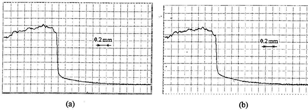
Fig.36. Reconstructed image of the sharp edge without distortions, reading out in green (a) and red (b) spectral bands (see Fig.4.).
