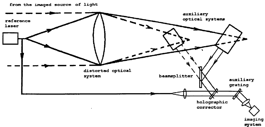
Fig.2. Optical scheme of the nonreciprocal imaging system with the holographic correction for distortions.
