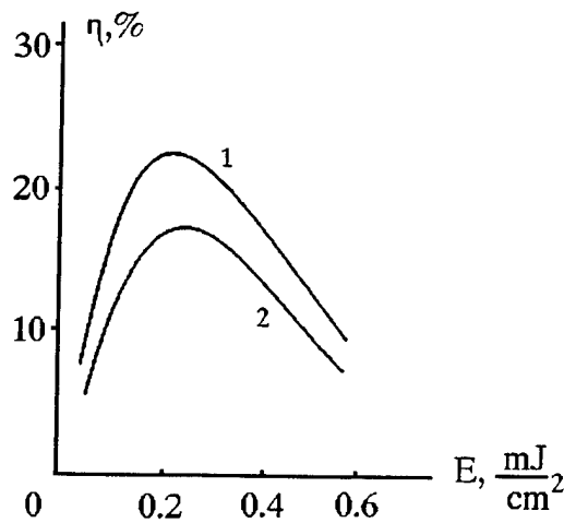
Fig.38. Peak values of DE vs. radiation energy fluency without distorter (1) and with the distorter 0.006 radian (2).
