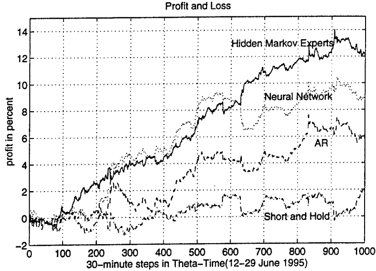
Figure 3: Profit and Loss for Olsen data. This figure shows that the Hidden Markov Experts give the highest profit in comparison to the pure linear regression and the feed-forward neural network. Transaction cost are not taken into account.
