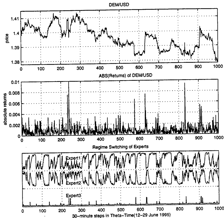
Figure 2: Panel 1 of this figure is the test set of the Olsen data. Panel 2 shows the absolute values of the return of the price. Panel 3 shows the regimes found by each experts for the Olsen data. We plot the responses of all three experts in this panel with different offsets. We can see that the first expert is responsible for the low volatility regions, while the second expert is responsible for high volatility regions, and the third expert acts as a collector for the outliers. This result is consistent with the variances of each expert, given in Figure 4.
