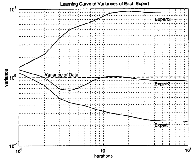
Figure 4: Learning curve of the variance for each expert for the Olsen data. We can see that the first expert is responsible for the low volatility regions, while the second expert is responsible for high volatility regions (similar to the variance of the time series). The third expert acts as a collector for the outliers. (The data is normalized to unit variance.)
