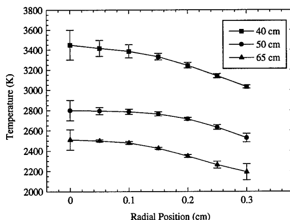
Figure 20. Temperature profiles of the air/argon plasma at 40, 50, and 65 cm downstream of nozzle exit.
