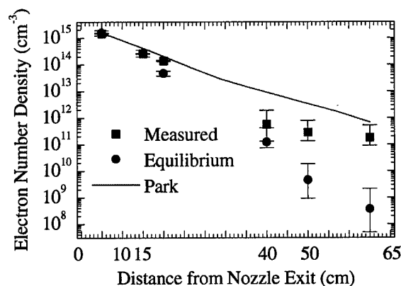
Figure 28. Electron number densities in the air/argon plasma.
