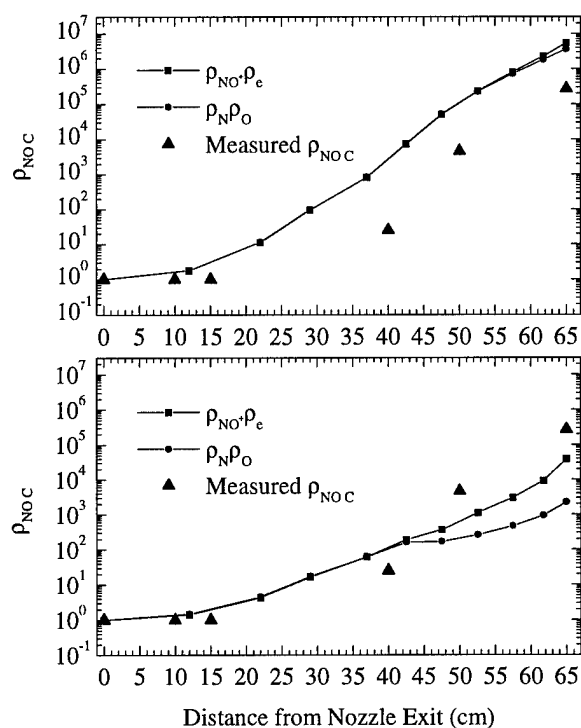
Figure 26. Comparison between calculated and measured NO C state nonequilibrium factors. Top frame (26a) uses Park's mechanism. Bottom frame (26b) uses Park's mechanism with a rate of NO thermal dissociation enhanced by a factor 10.
