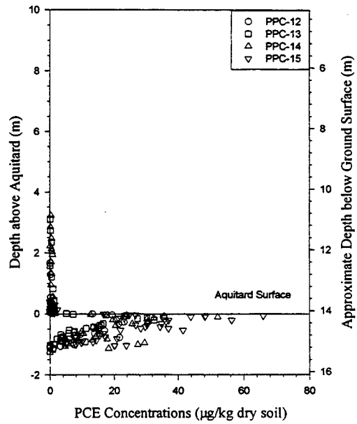
Figure 25. Initial and Final PCE Concentrations in CPC and PPC (Core Data).
