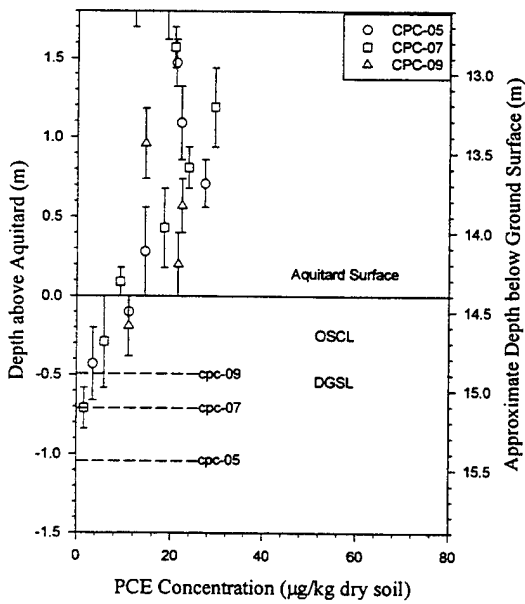
Figure F-2. Results of Prepumping and Postpumping Concentrations of TCE (top) and PCE (bottom) in Selected Mid-Cell CPC Soil Cores. (Prepumping data are on the left; postpumping data are on the right).
