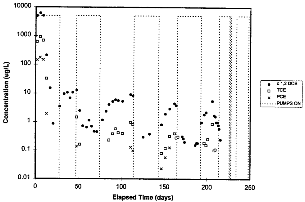
Figure G-6. Selected Elution Curves for the Sampling Point PP-ML-8-2. Dashed lines show when pumping occurred.
