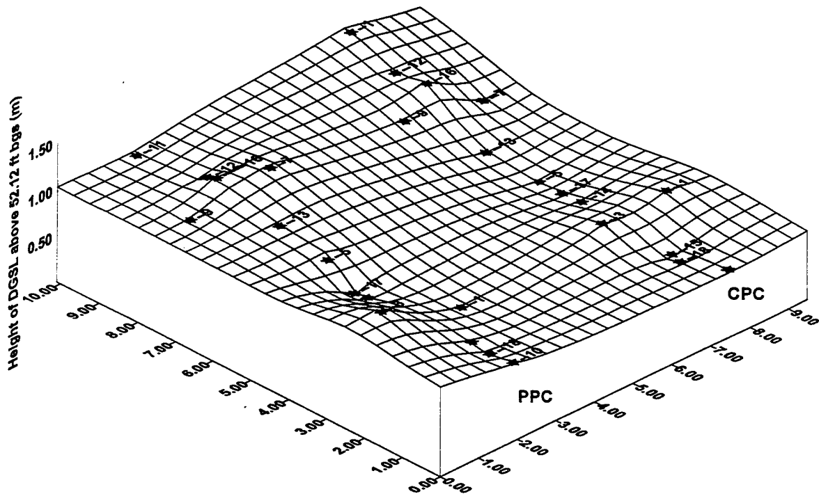
Figure H-1 Surface Contour Map of OSCL and DGSL Layers (Unmarked locations in bottom figure did not contain the DGSL interface)
