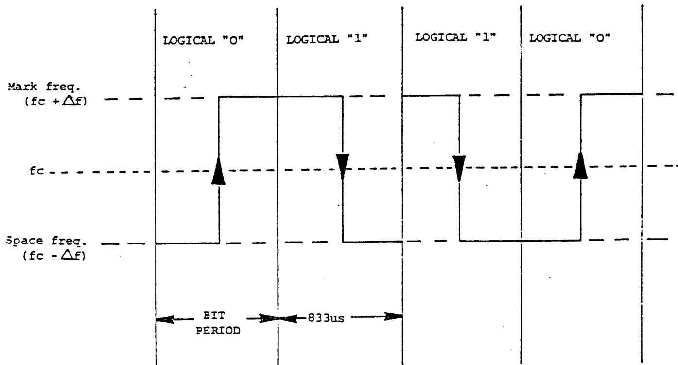
FIGURE 6 MANCHESTER CODING
