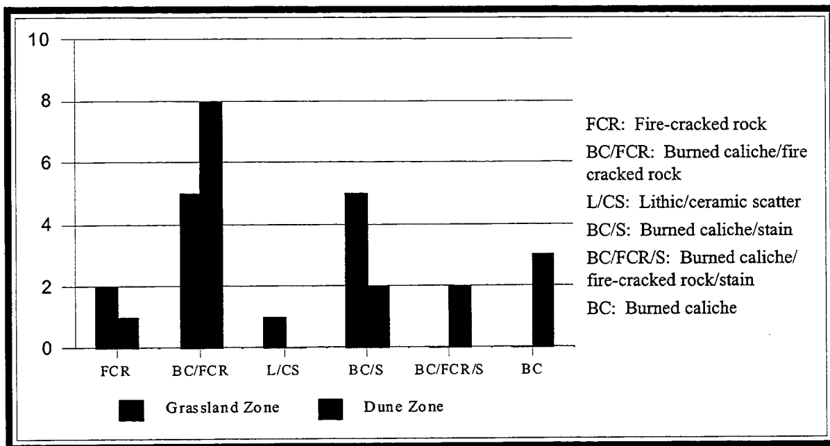
Figure 4.2. Grassland and Dune Zone Features.
