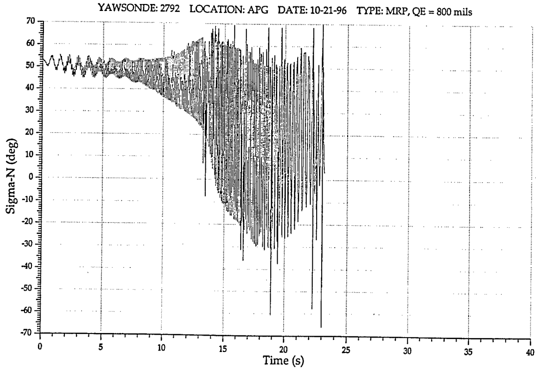
Figure 29: Spin Decay (top) and Yaw History (bottom) of MRP #3
