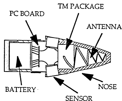
Figure 19: Yawsonde Schematic
