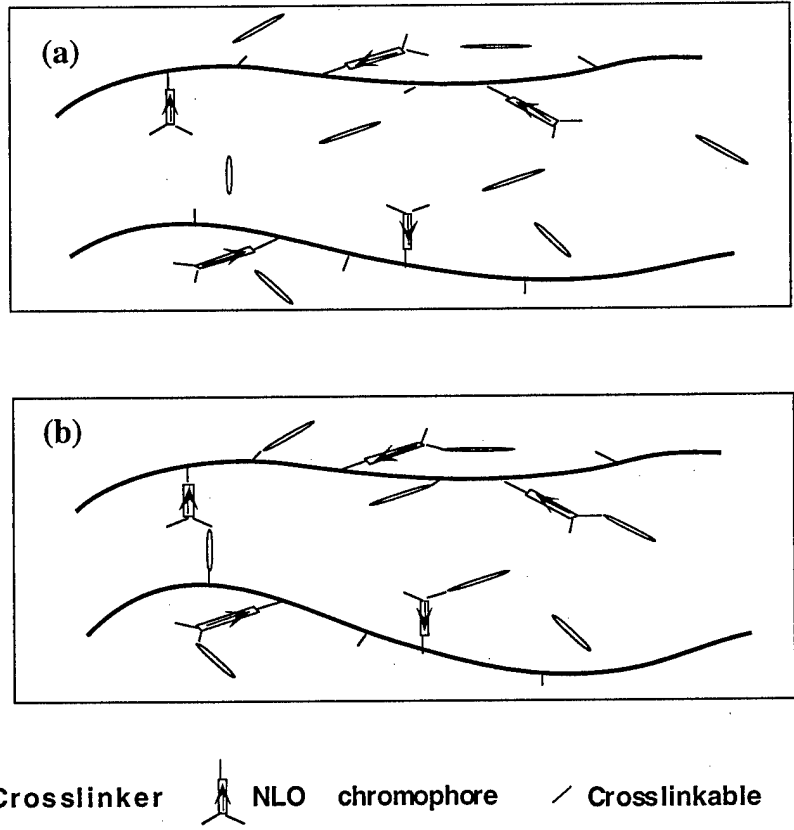
FIGURE 2.3. Mechanism of anchoring the crosslinker. (a) free crosslinker can diffuse and crystallize out; (b) slow evaporation rate allows a crosslinker to have time to attach one end to the polymer backbone, but the second end of a chromophore has much less chance to encounter a crosslinkable site.
