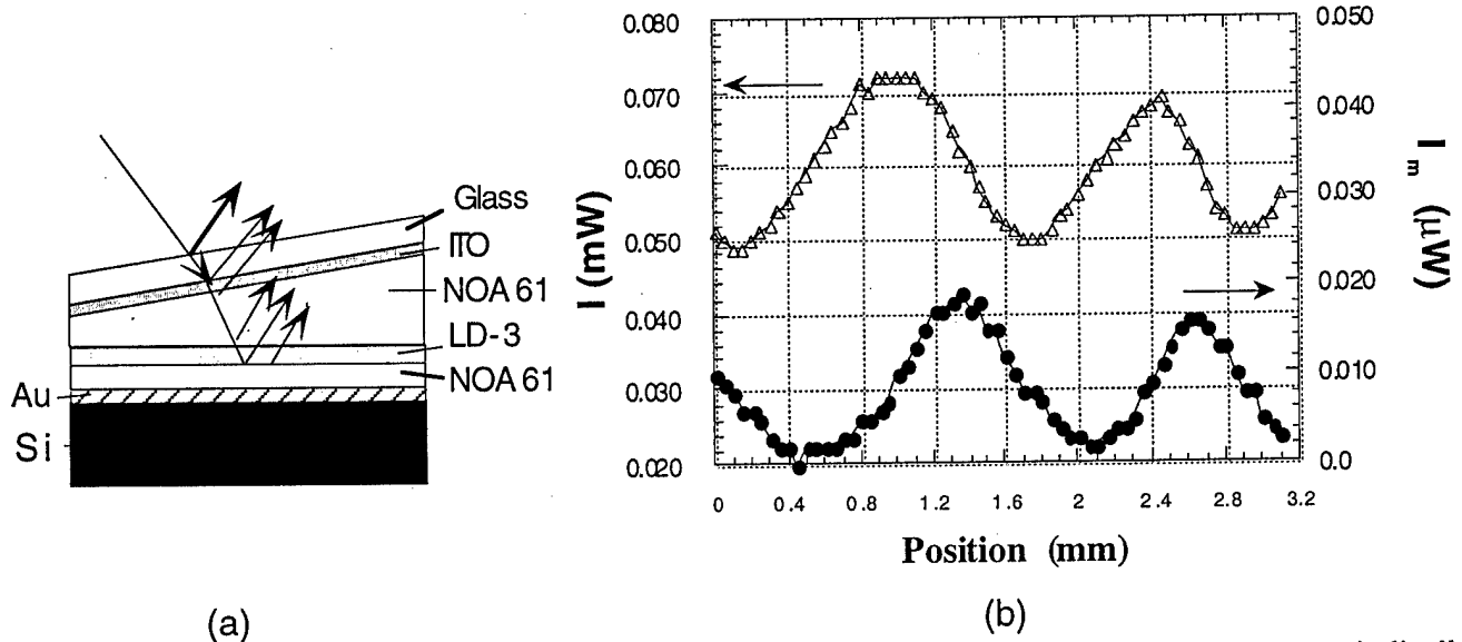
FIGURE 3.2. The reflected light intensity I and the modulated signal I_m both change in value periodically with increases in the top-cladding thickness. (a) A schematic of the sample with varying top-cladding thickness and (b) measured I and I_m curves
