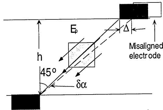
FIGURE 4.5 The effect of misaligned electrode on the tiltness of poling field
