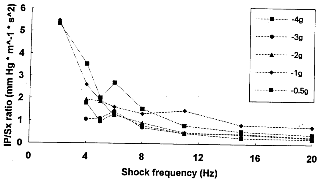
Figure F-84. Internal pressure response to seat x acceleration for -0.5, -1, -2, -3, and -4 g shocks.
