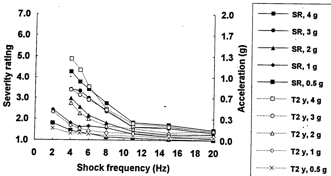
Figure F-115B. Comparison between severity ratings (SR) and acceleration measured at the thoracic spine (T2) in response to positive y axis shocks (T2 y).
