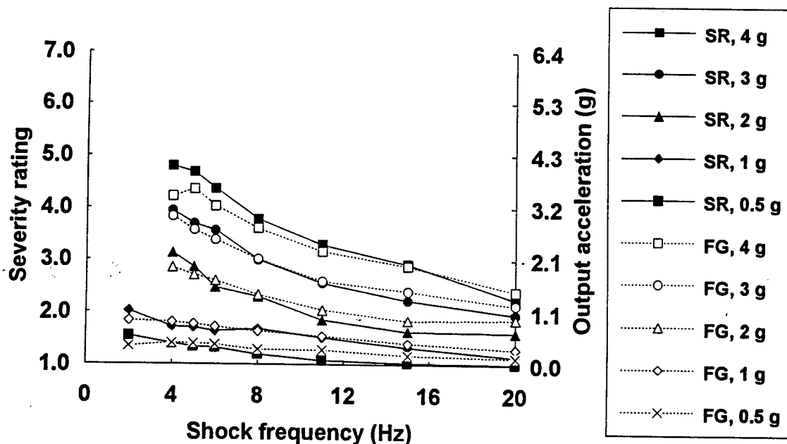
Figure F-98. Comparison between severity ratings (SR) and expected output from the Fairley-Griffin (FG) model to positive z axis shocks.
