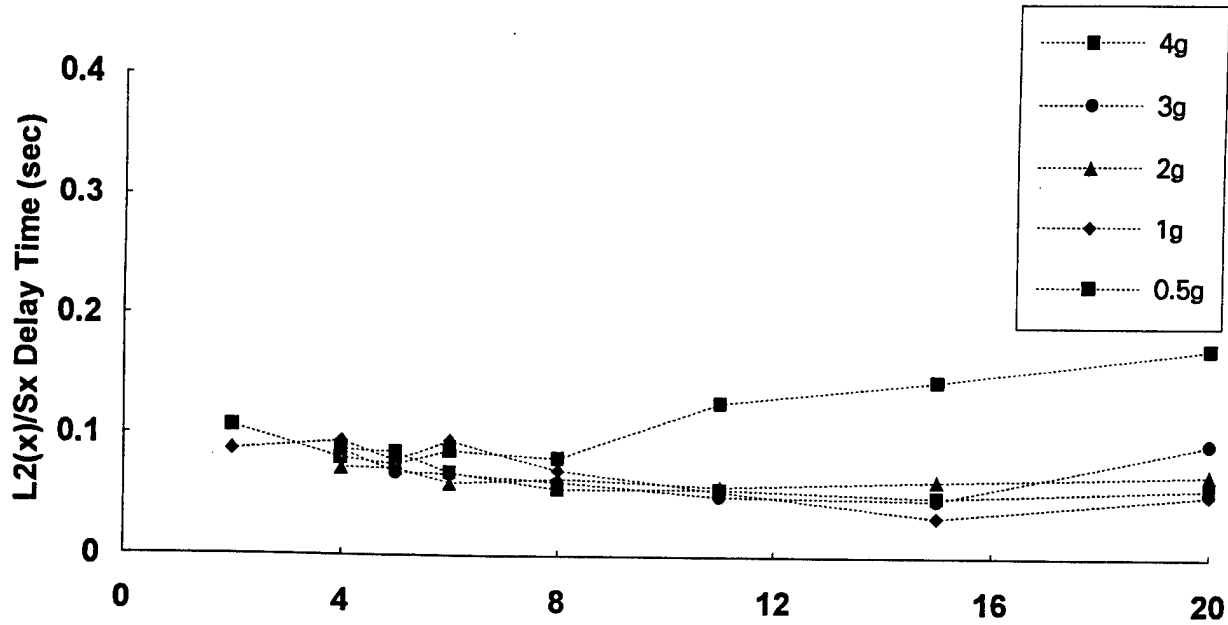
Figure F-69. Delay time for peak acceleration measured at spine (L2) to seat x acceleration for -0.5, -1, -2, -3, and -4 g shocks.
