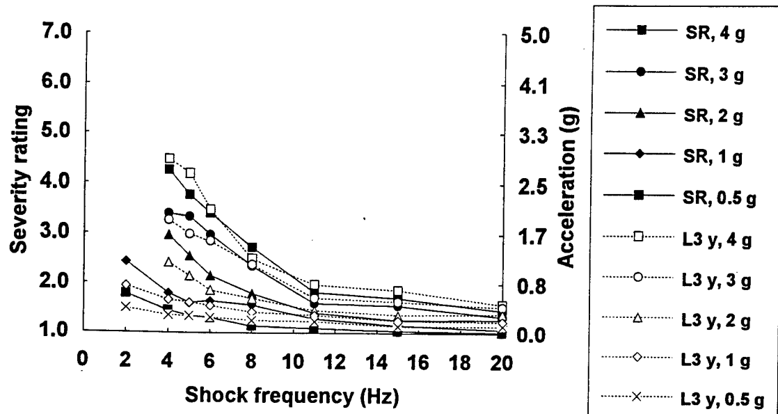
Figure F-115C. Comparison between severity ratings (SR) and acceleration measured at the lumbar spine (L3) in response to positive y axis shocks (L3 y).
