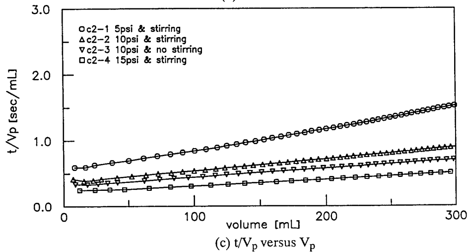
Figure 41. Effects of pressure on flux of sample #3 (MF 0.22\mu\text{m} ).
