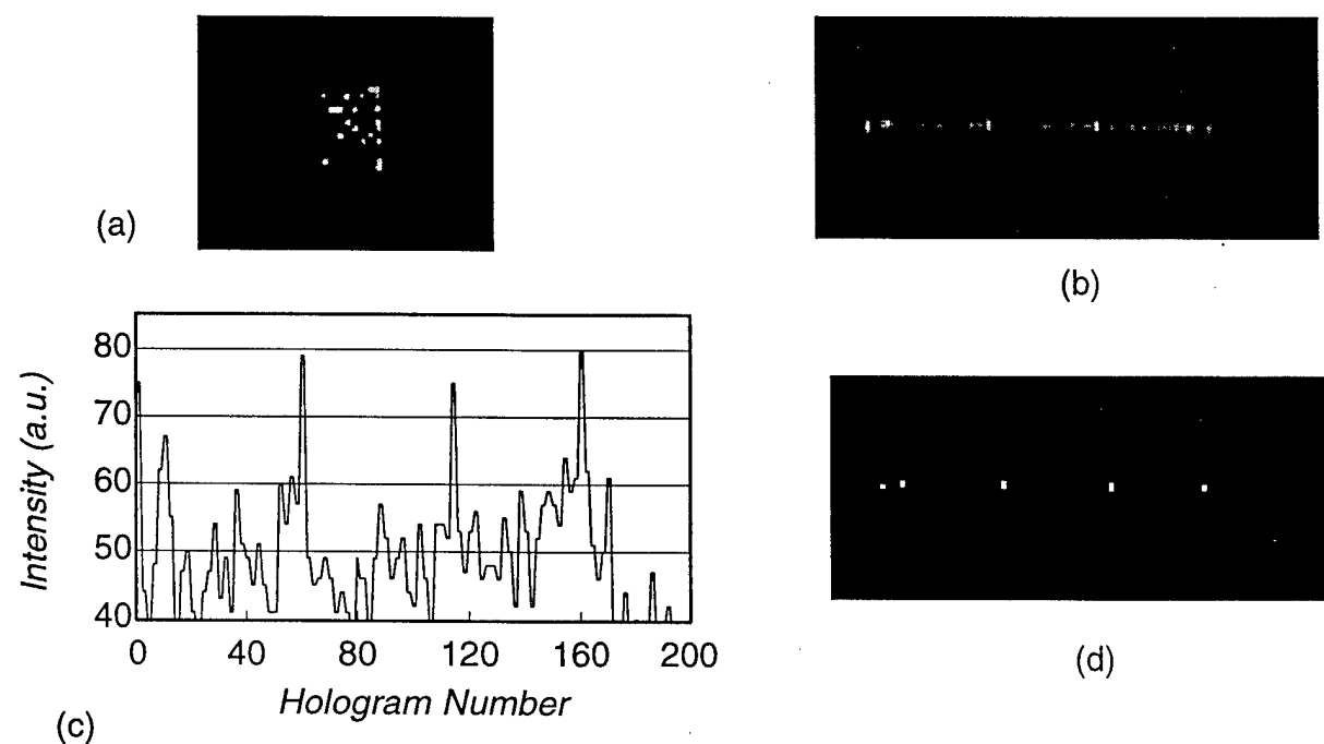
Figure 23: (a) Search argument, 1/30 of a data page, (b) Reconstructed reference plane, (c) Intensity profile along the center of the reconstruction, and (d) Thresholded reconstruction.
