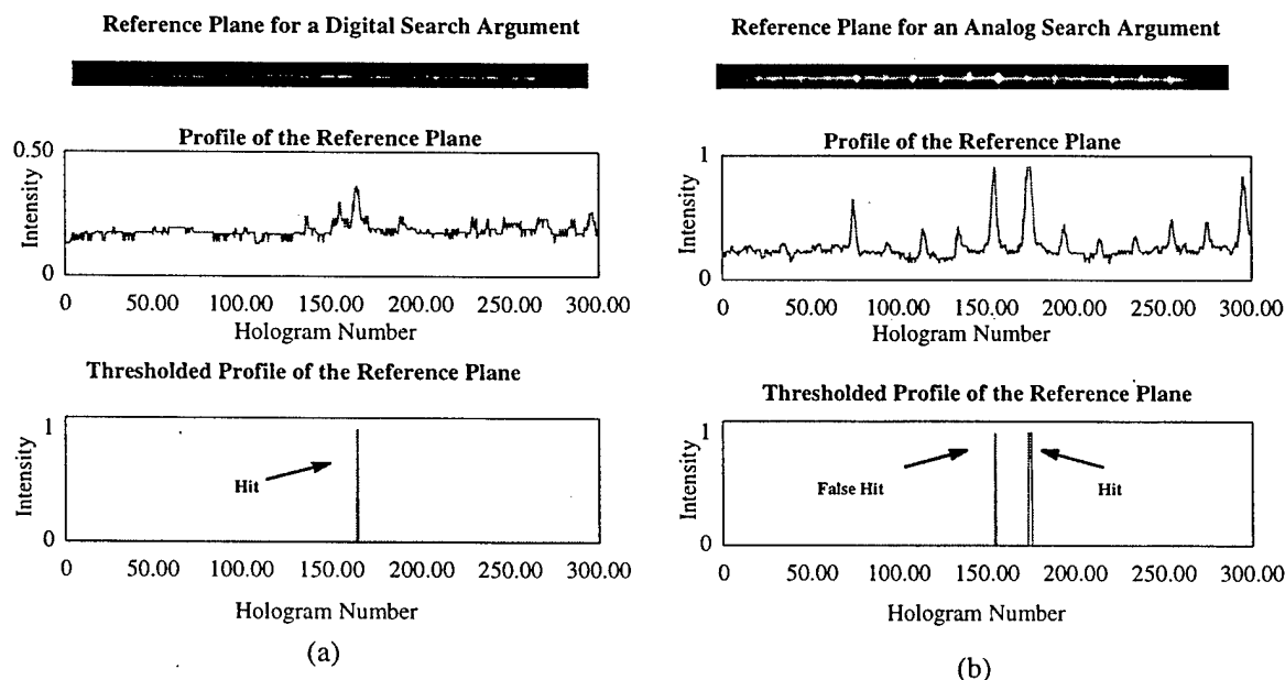
Figure 34. Associative recall of (a) a digital and (b) an analog data page.
