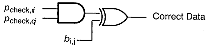
Figure 11: Bit correction hardware.
