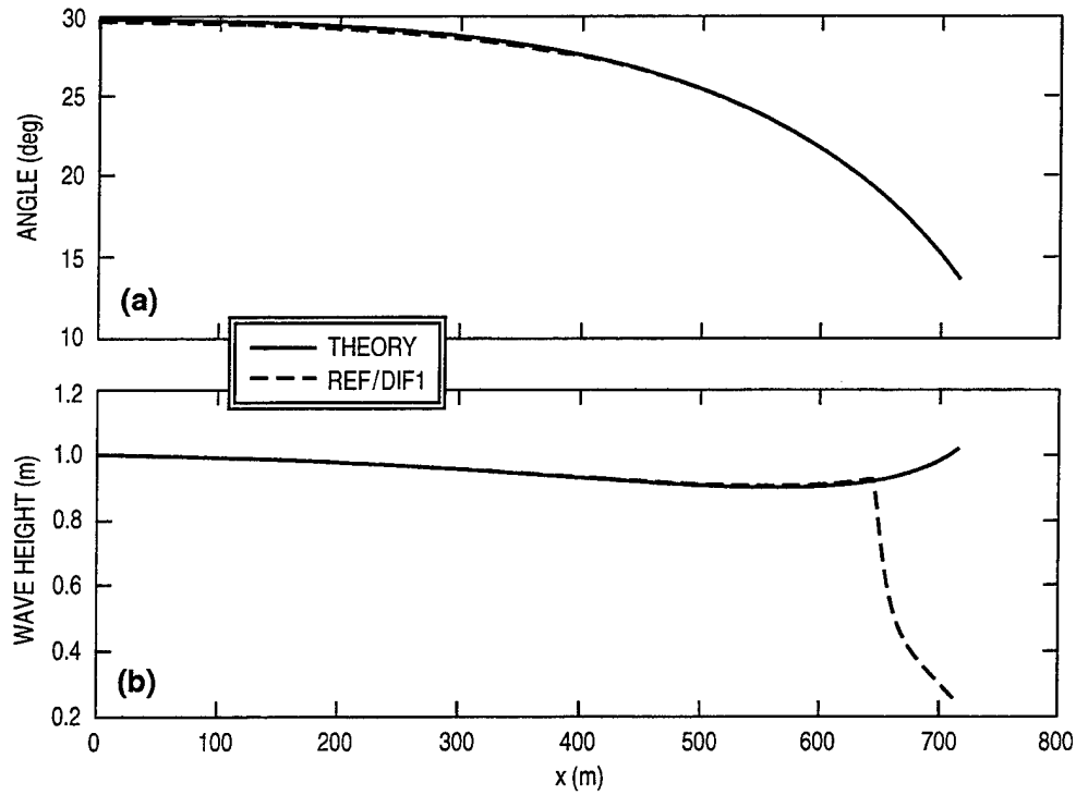
Fig. 2 — Comparison between model results and linear theory for refraction/shoaling test, (a) wave angle comparison and (b) wave height comparison. Wave period = 3 s, angle = 30^\circ .
