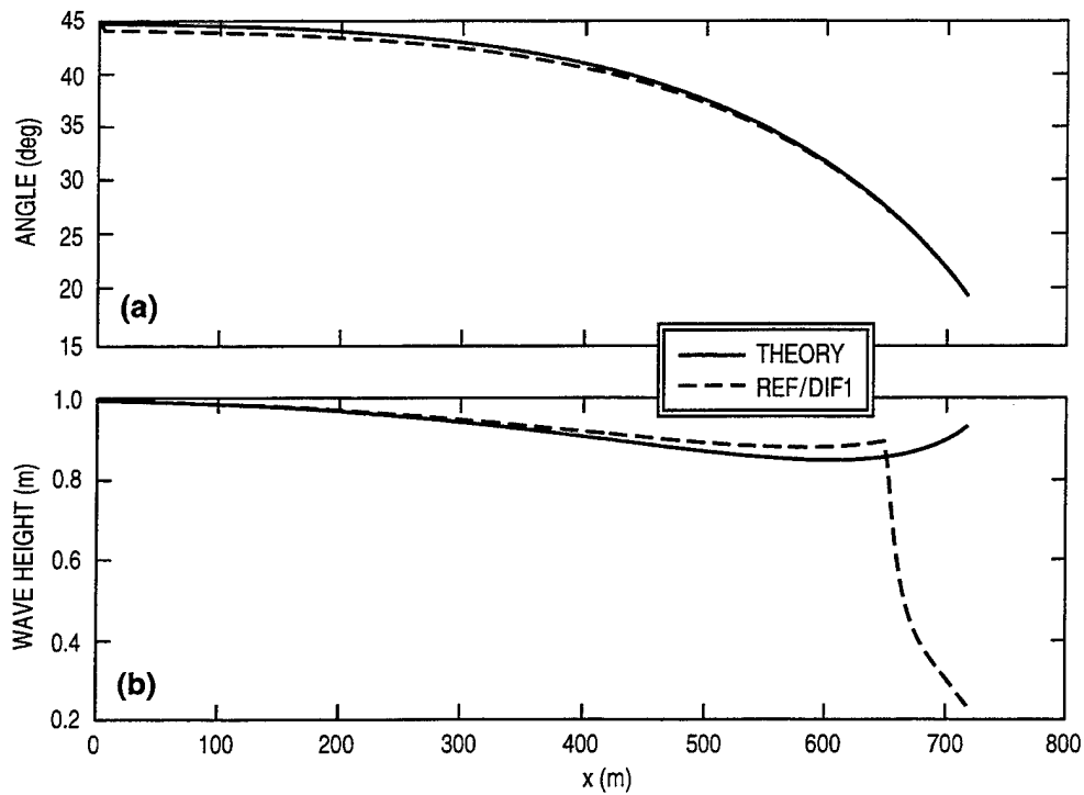
Fig. 3 — Comparison between model results and linear theory for refraction/shoaling test, (a) wave angle comparison and (b) wave height comparison. Wave period = 3 s, angle = 45^\circ .
