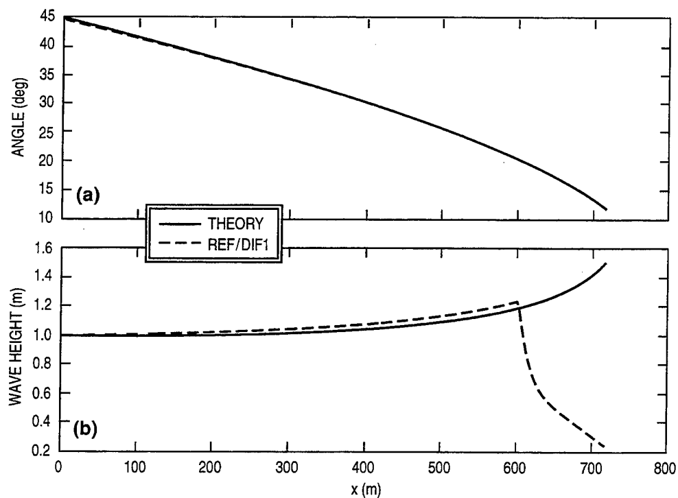
Fig. 7 — Comparison between model results and linear theory for refraction/shoaling test, (a) wave angle comparison and (b) wave height comparison. Wave period = 10 s, angle = 45°.
