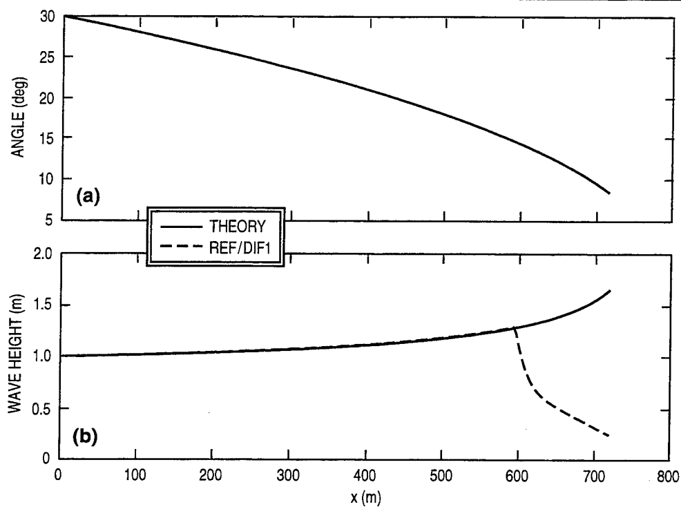
Fig. 6 — Comparison between model results and linear theory for refraction/shoaling test, (a) wave angle comparison and (b) wave height comparison. Wave period = 10 s, angle = 30°.
