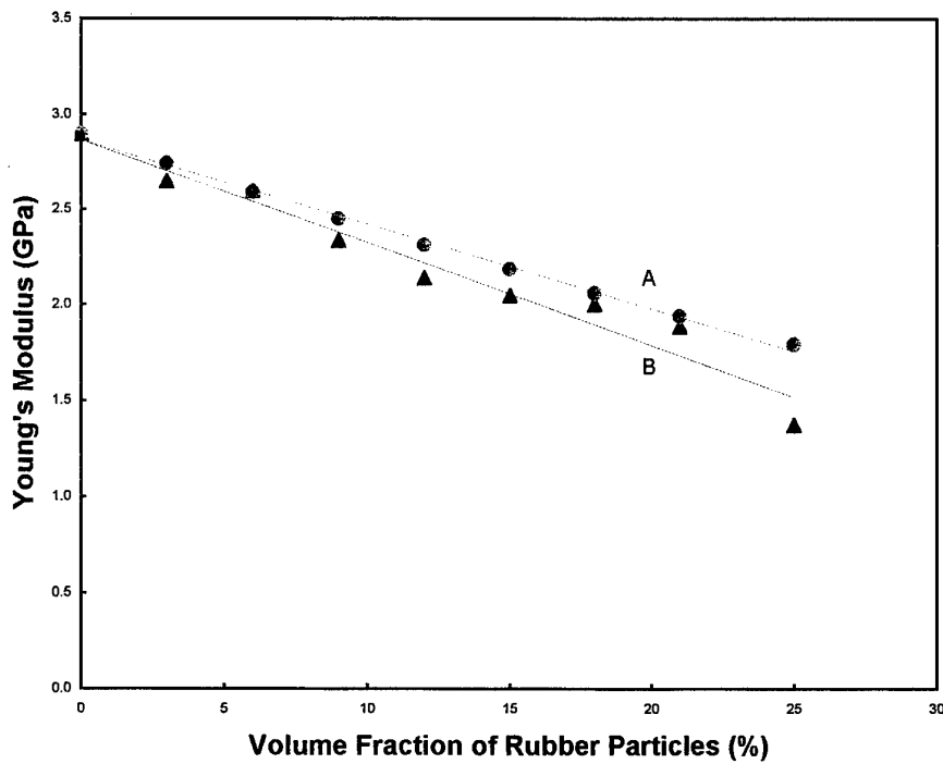
Figure 12 Young's modulus for epoxy/rubber composites as a function of volume fraction ( \phi ) of rubber particles. Lines B is the data and Line A is from a literature model.
