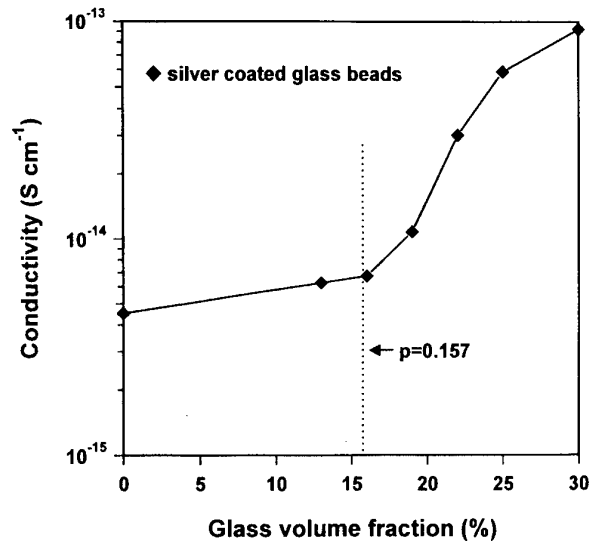
Figure 1 Demonstration that the system glass beads/epoxy resin conforms to a percolation model (conductivity measurements using silver-coated beads).
