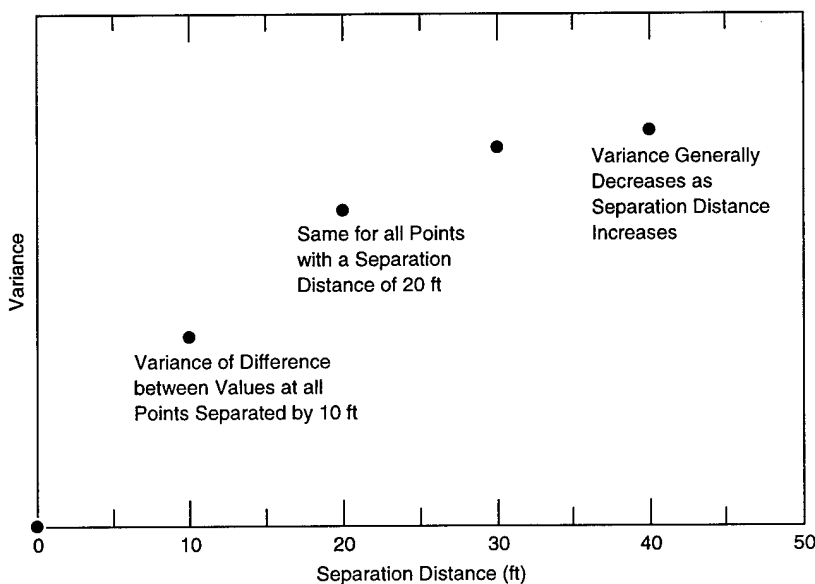
b. Variogram development.
