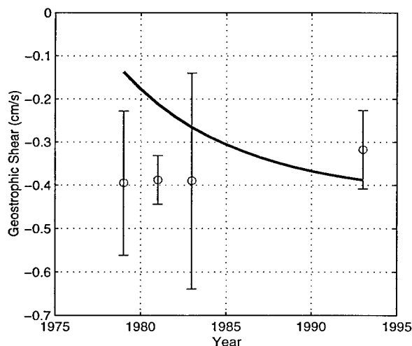
Figure 3.8: Meridional geostrophic velocity shear between 250 and 500 dbar centered at 26^\circ\text{N} , 30^\circ\text{W} . Error bars represent 95% confidence intervals. For comparison, the solid line shows implied shear from evolution of tracer age signal.
