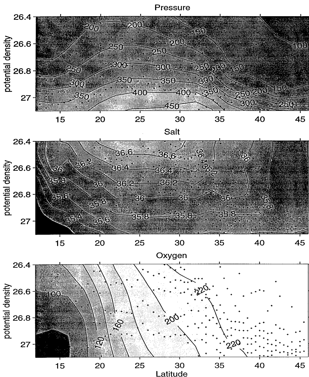
Figure 2.4: Vertical sections of properties along nominal 25°W: a) Pressure (dbar) b) Salinity (psu) and c) Oxygen \mu\text{mol} - \text{kg}^{-3} . Gridded fields were obtained by objectively mapping the measurements with a Gaussian correlation function with characteristics scales of three degrees in the horizontal and 0.25 \text{ kg} - \text{m}^{-1} in the vertical.
