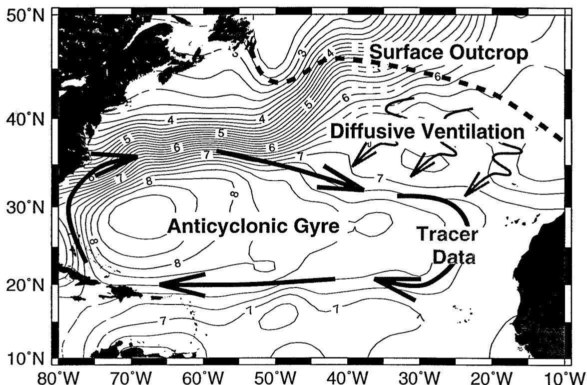
Figure 5.15: Schematic of implied ventilation on \sigma_\theta = 27.0 . Contours show the isopleths of the pressure anomaly Montgomery streamfunction referenced to \sigma_1 = 32.3 .
