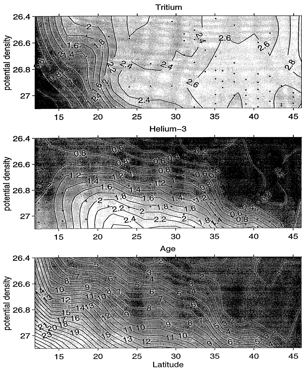
Figure 2.5: Vertical sections of transient tracer fields along 25°W. a) Tritium (T.U.) b) ^3\text{He} (T.U.) and c) tritium- ^3\text{He} age (years) sections along nominal 25°W. Position of ^3\text{H} and ^3\text{He} samples are indicated by small crosses. Age is calculated from the grided fields of ^3\text{H} and ^3\text{He} .
