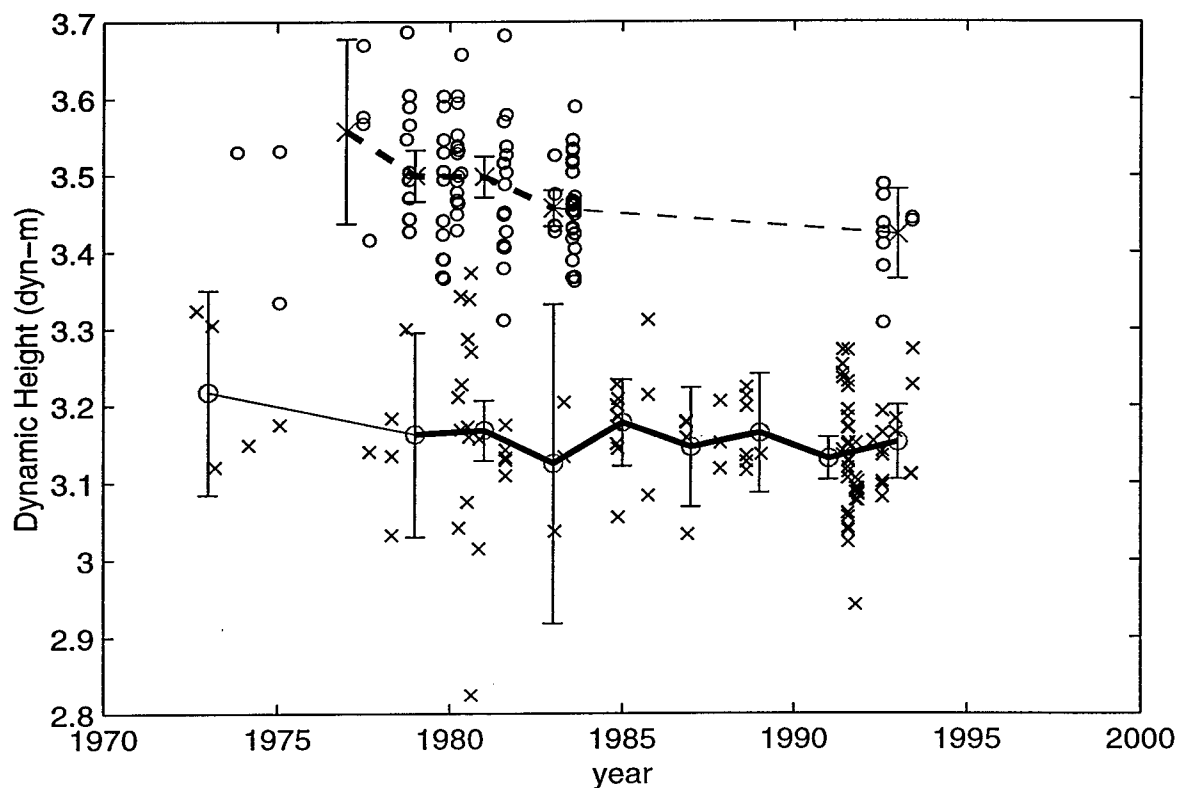
Figure 3.7: Time series of dynamic height at 250 dbar referenced to 500 dbar to two points centered at 26^{\circ}\text{N} , 36^{\circ}\text{W} (o) and 26^{\circ}\text{N} , 24^{\circ}\text{W} (x). Solid and dashed lines display mean values, with 95% confidence intervals, calculated from two year bins of the data time series.
