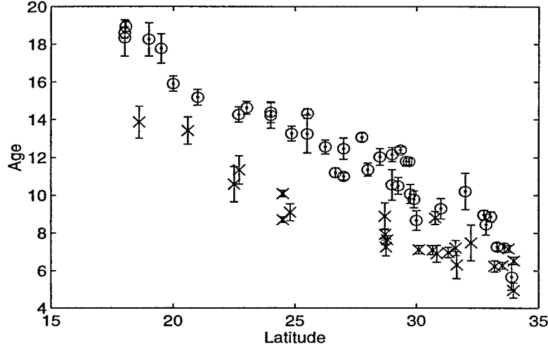
Figure 2.19: Tritium- 3 He age on \sigma_\theta = 27.0 at two different years. Samples collected in 1992 are indicated by a 'o' while those from 1981 are represented with an 'x'. Error bars represent uncertainty to the combined analytic and interpolation errors.
