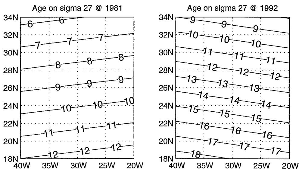
Figure 2.18: Two realizations of the tritium- ^3\text{He} age field on \sigma_\theta = 27.0 as determined by the time-dependent regression model. Left-hand figure shows age field in 1981 and right-hand figure shows age in 1992
