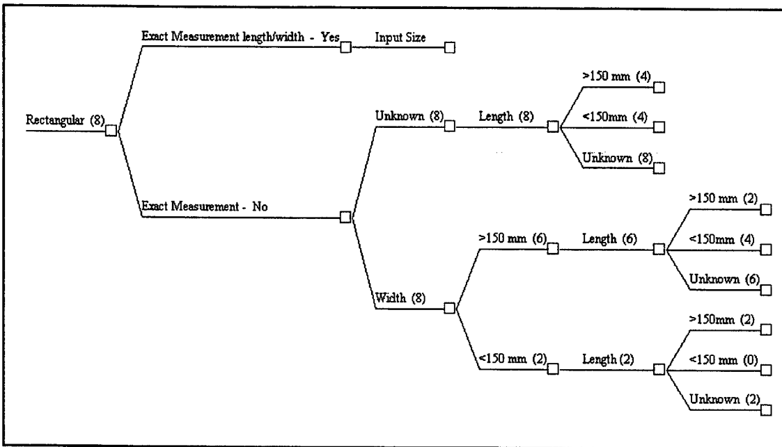
Figure 3.4 Rectangular Size Question Tree
