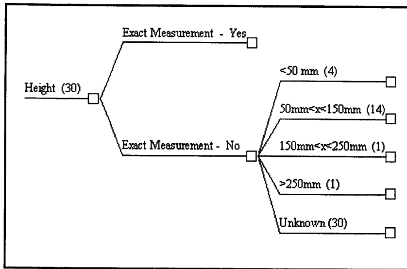
Figure 3.7 Height Question Tree
