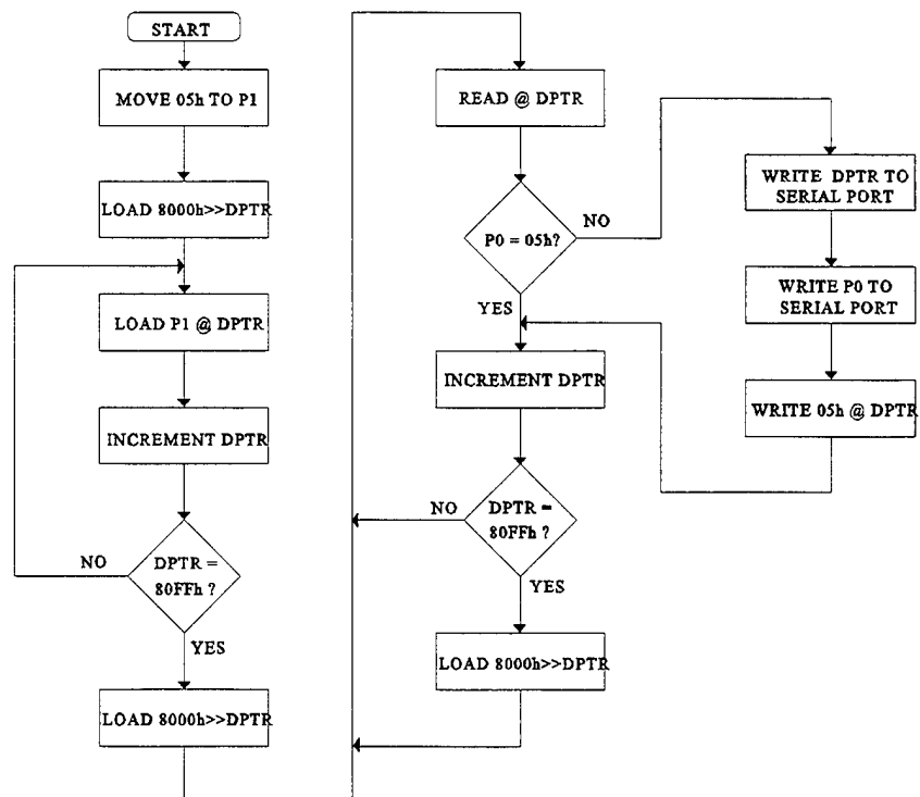
Figure 7.4 Flow Chart for Vitesse SRAM
