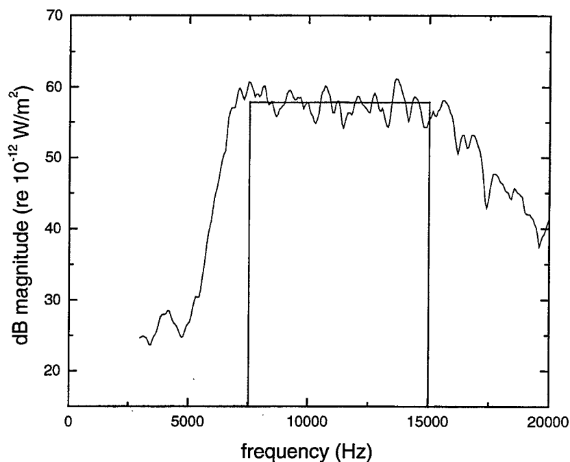
Figure 4.4. Ideal ("brick wall") 7.5 - 15 kHz spectrum compared to actual 7.4 - 15.3 kHz spectrum showing less structure and a flatter spectral shape. The total intensity of the noise corresponds to 133.5 dB (re 10^{-12} W/m 2 ).
