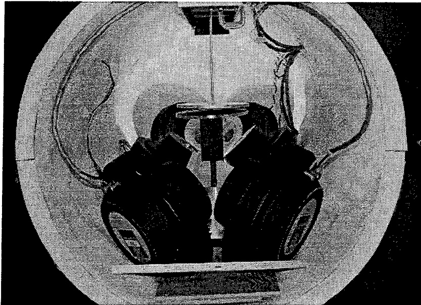
Figure 4.1. Internal view of acoustic Chamber showing equipment arrangement. The step motor mount is 48 cm from the open end.
