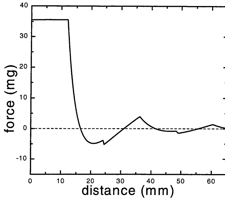
Figure 2.2. Plot of the force between two parallel rigid plates, 15 cm in diameter, as a function of the separation between them, Eq (2.11). The force is due to the radiation pressure of flat noise between 7.5 kHz -15 kHz. The total intensity of the noise is 133 dB (re 10^{-12} W/m 2 ).
