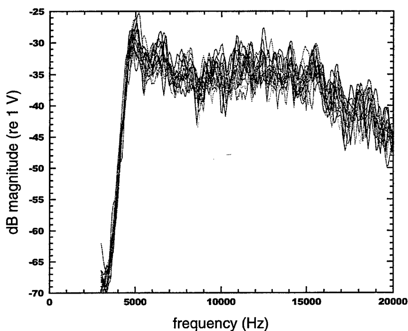
Figure 3.4. Acoustic field intensity measurements for horizontal locations 34-44-54 cm measured left/right and vertical(high/low/center) for 5 kHz to 20 kHz. The spectrum is essential flat from 5 kHz to 15 kHz, rolling off 20 dB from 15 to 20 kHz.
