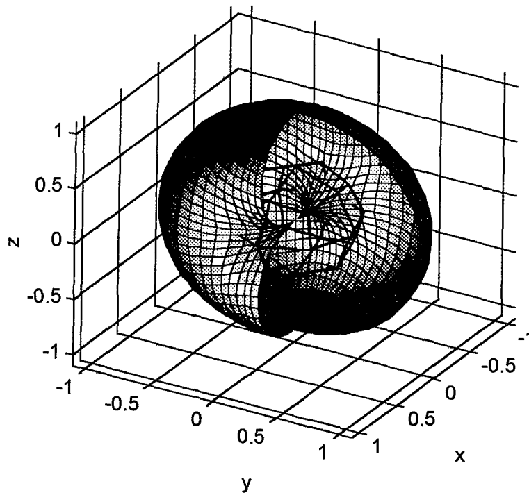
Figure (Fig. A-19), Total electric field pattern for the sphere's first eigen frequency with cut out
