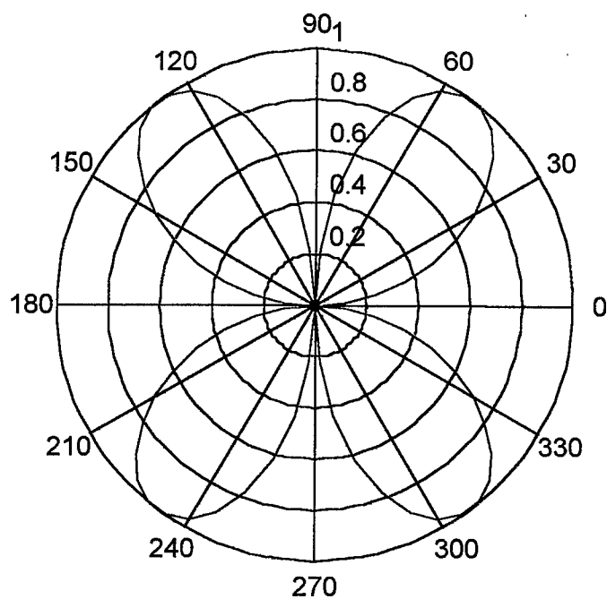
Figure (Fig. A-13), YZ plane polar plot for the thin wire model at 143.9 MHz
