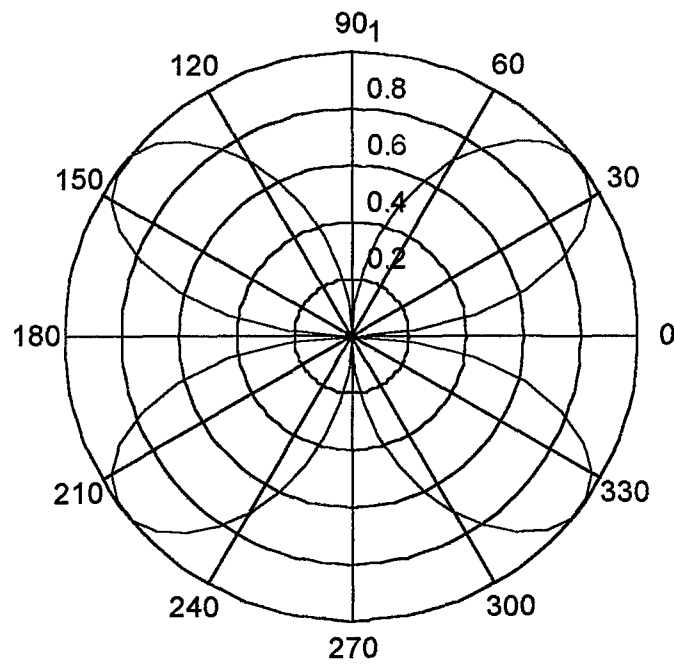
Figure (Fig. A-11), XZ plane polar plot for the thin wire model at 143.9 MHz
