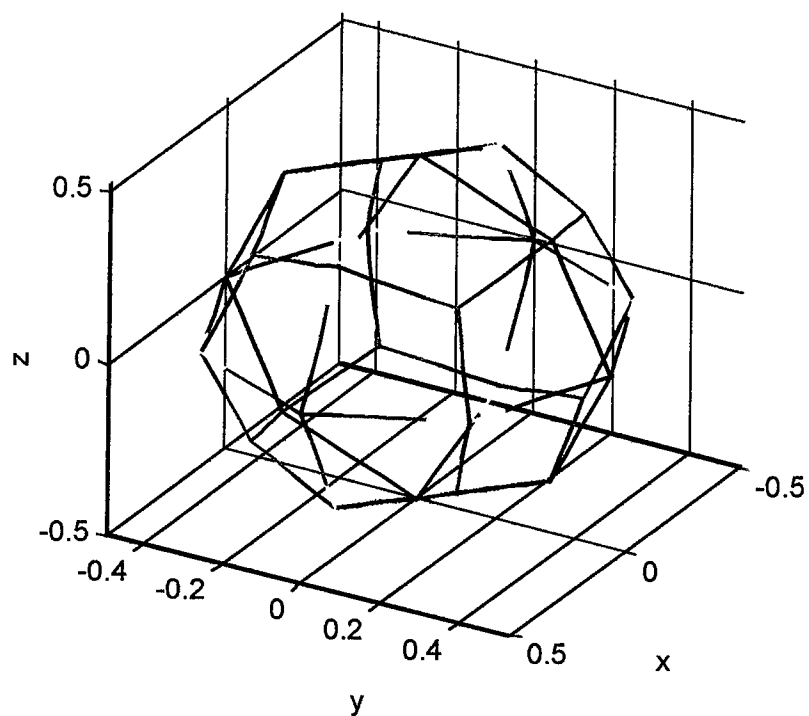
Figure (Fig. A-17), Current density for the first eigen frequency for the sphere
