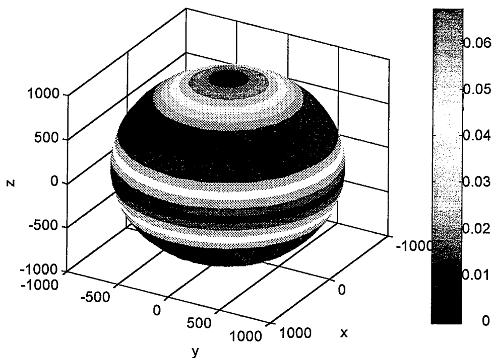
Figure (Fig. A-15), Field magnitude of thin wire model at 143.9 MHz and at a distance of 1000 m
