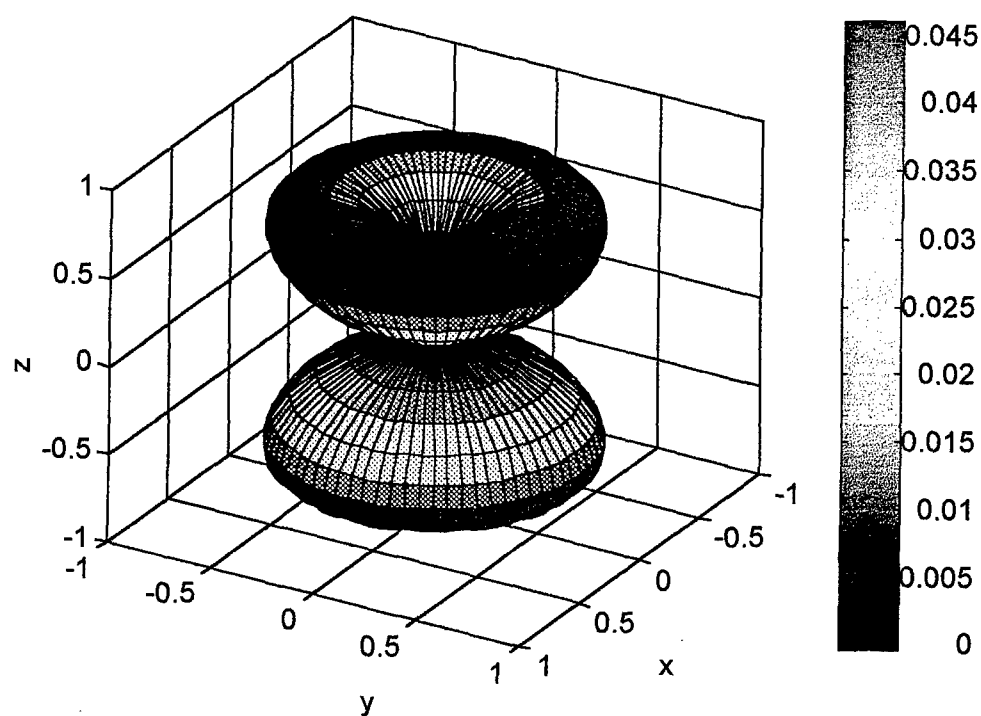
Figure (Fig. A-7), Horizontal field magnitude for the thin wire model at 143.9 MHz
