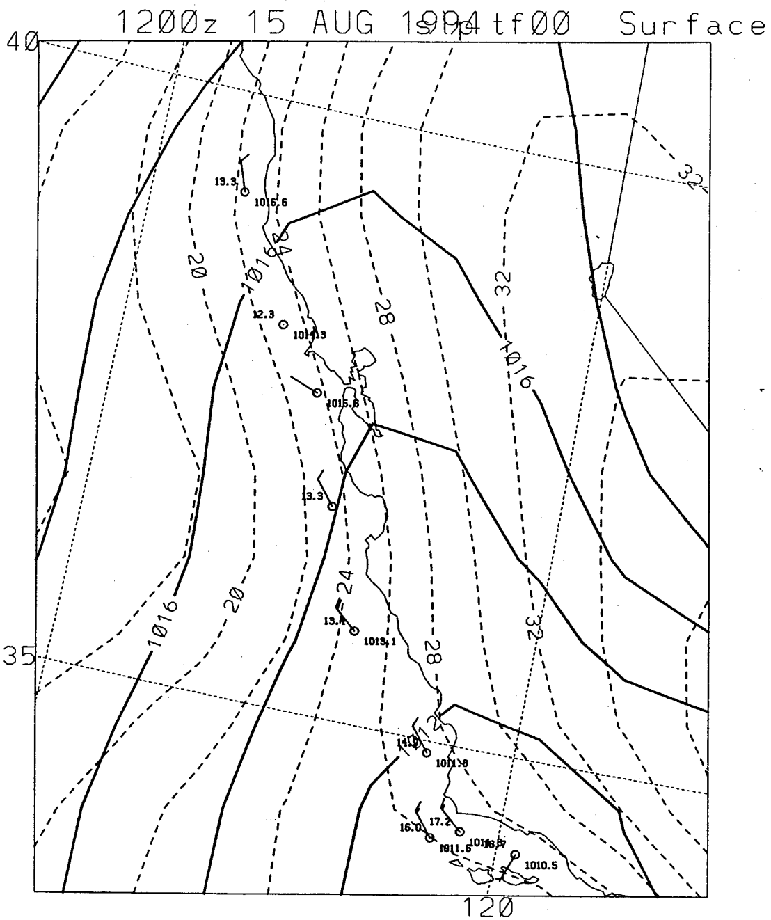
Figure 9. Surface synoptic chart for August 15, 1994 (1200 UTC)
