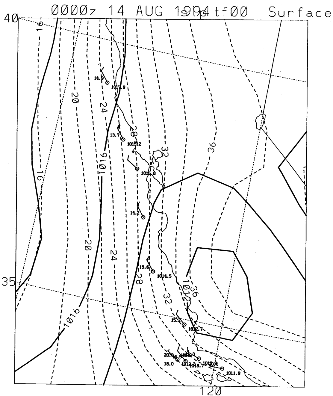
Figure 3. Synoptic surface analysis for August 14, 1994 (0000 UTC)
