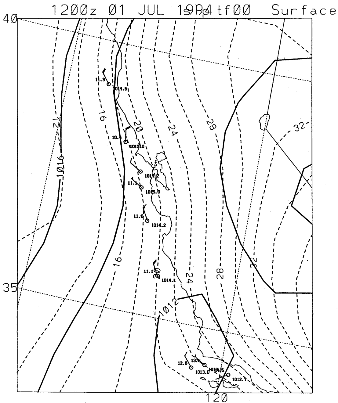
Figure 5. Synoptic surface analysis for July 01, 1994
