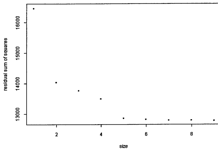
Figure 7. Variable Selection via Stepwise Regression.
