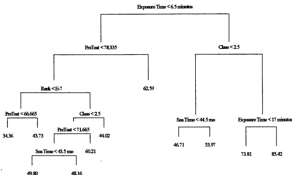
Figure 8. Tree-based model (Complete data set).
