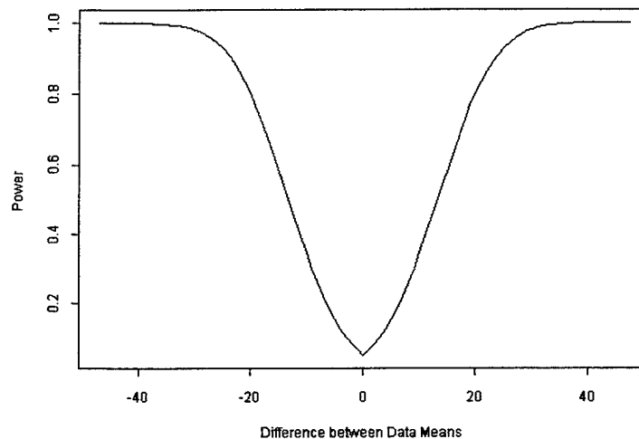
Figure 19. Power Function for May 97 Data Set.
