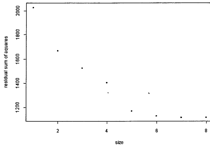
Figure 15. Variable Selection via Stepwise Regression.
