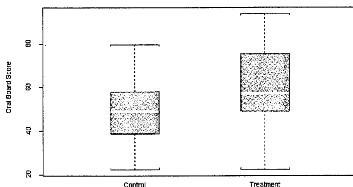
Figure 10. Boxplot comparison of Oral Board Scores (Complete Data Set).
