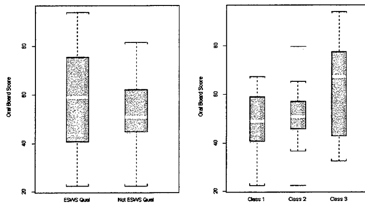
Figure 11. Boxplots of Complete Data Set variability.
