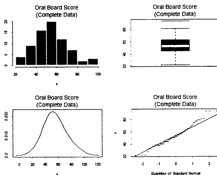
Figure 13. Diagnostic Plots for Complete Data Set.
