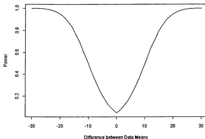
Figure 12. Power Function for Complete Data Set.
