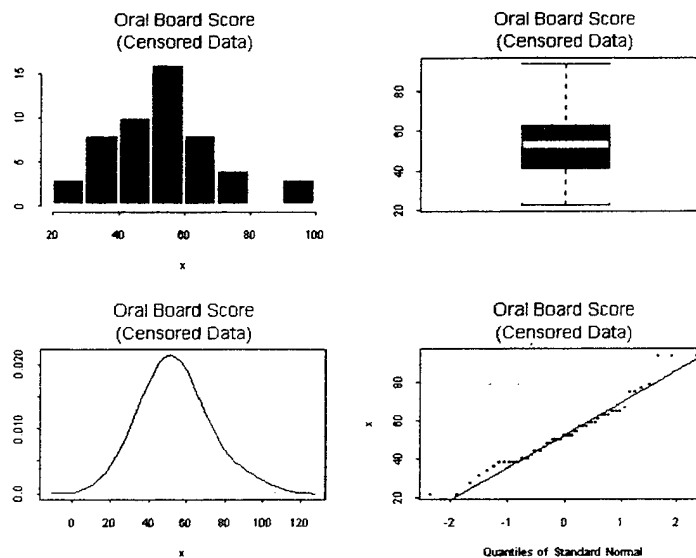
Figure 24. Diagnostic Plots for Censored Data Set.
