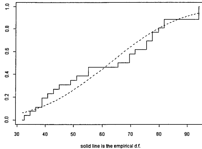
Figure 17. Empirical and Hypothesized Normal CDF's.
