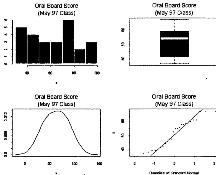
Figure 16. Diagnostic plots for the May 97 Class.
