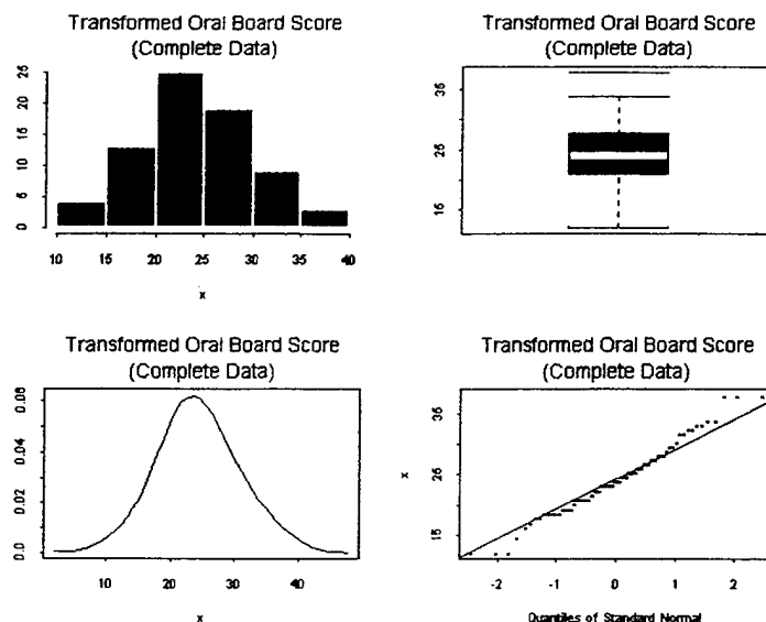
Figure 14. Diagnostic Plots for Transformed Data (Complete Data Set).
