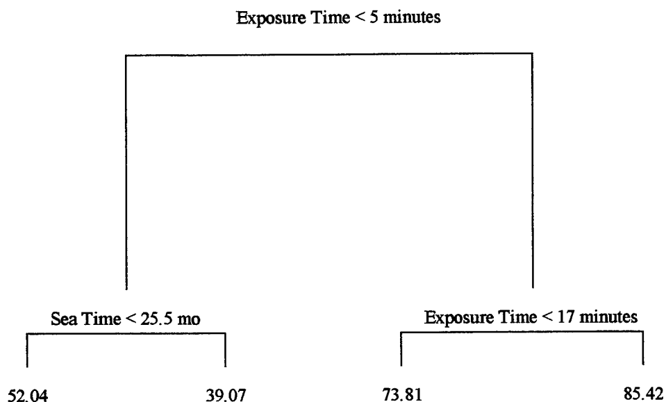
Figure 18. Tree-based model (May 97 class data set).
