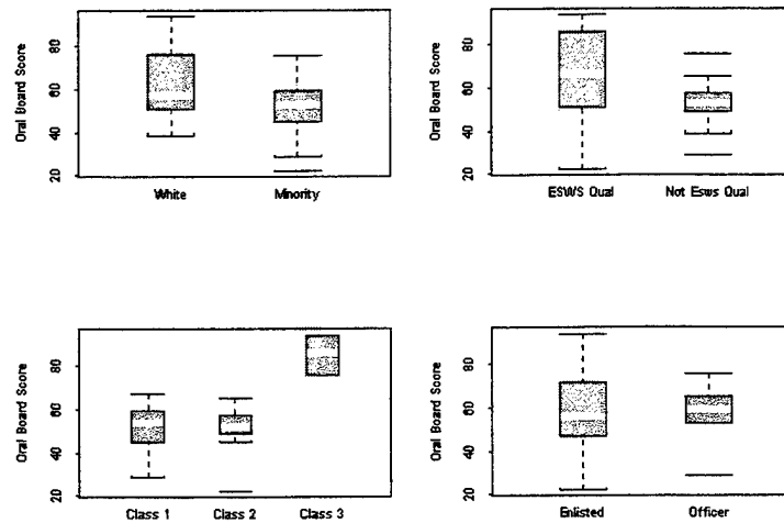
Figure 22. Boxplots of Treatment Group Variability.
