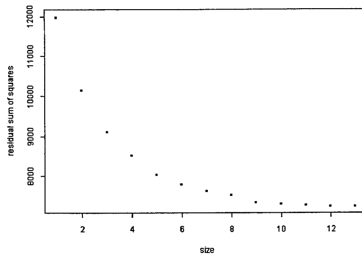
Figure 20. Variable Selection via Stepwise Regression.
