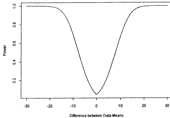
Figure 23. Power Function for Censored Data Set.
